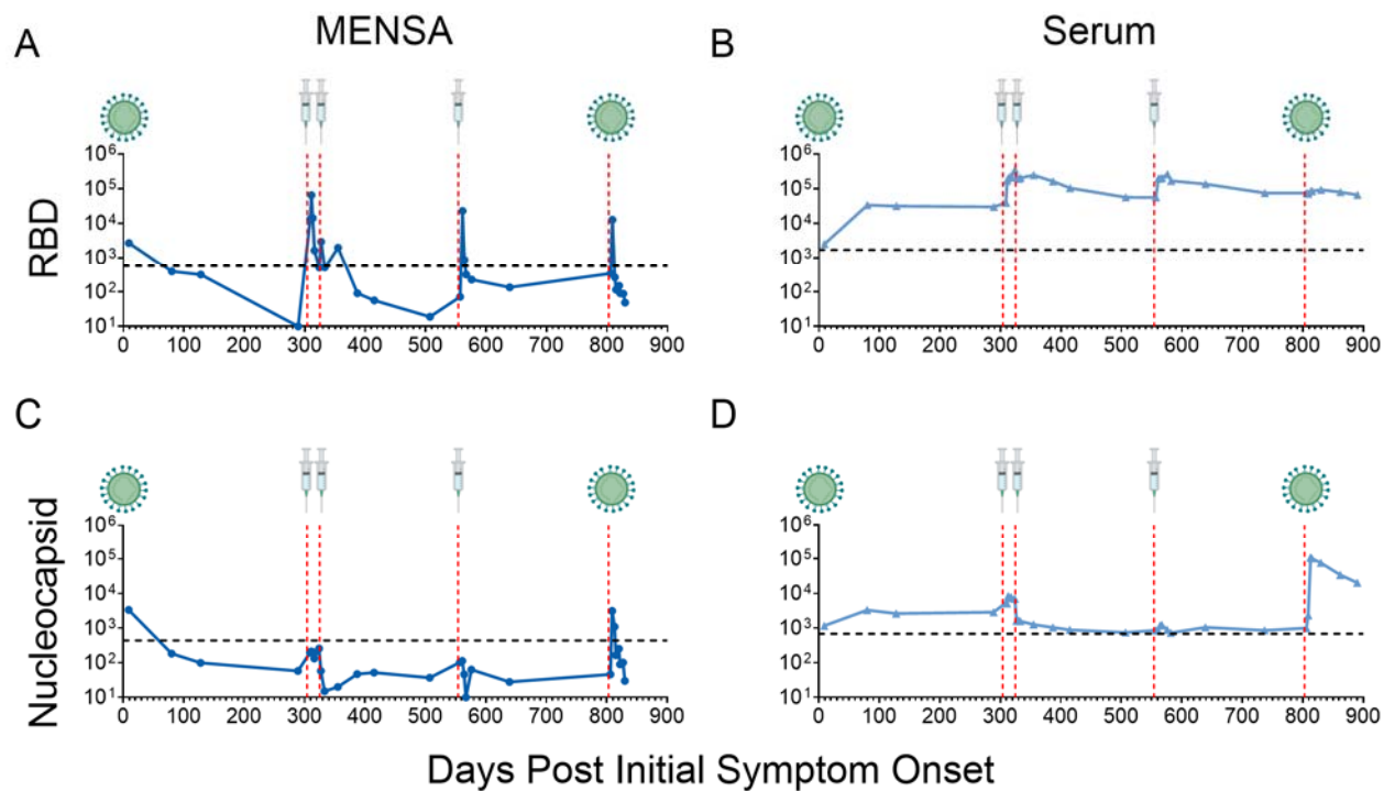
Figure 3. Kinetics of MENSEA and serum after SARS2 infection and multiple vaccine doses. Line graphs show MENSEA (dark blue) and serum (light blue) IgG antibody responses to S1-RBD (A,B) and Nucleocapsid (C,D) over time for a single patient starting with an initial primary SARS2 infection in 2020, through three doses of Pfizer COVID-19 mRNA vaccination in 2021, and a breakthrough Omicron infection in 2022. All values are reported as average Net MFI (Median Fluorescent Intensity – Background). Red vertical dashed lines represent a new exposure event. The primary and breakthrough infection events are symbolized as virions. Each vaccination dose event is symbolized as a syringe. Horizontal dashed black lines represent the C_0 threshold of positivity for each sample and antigen combination as determined from Figure 1.
