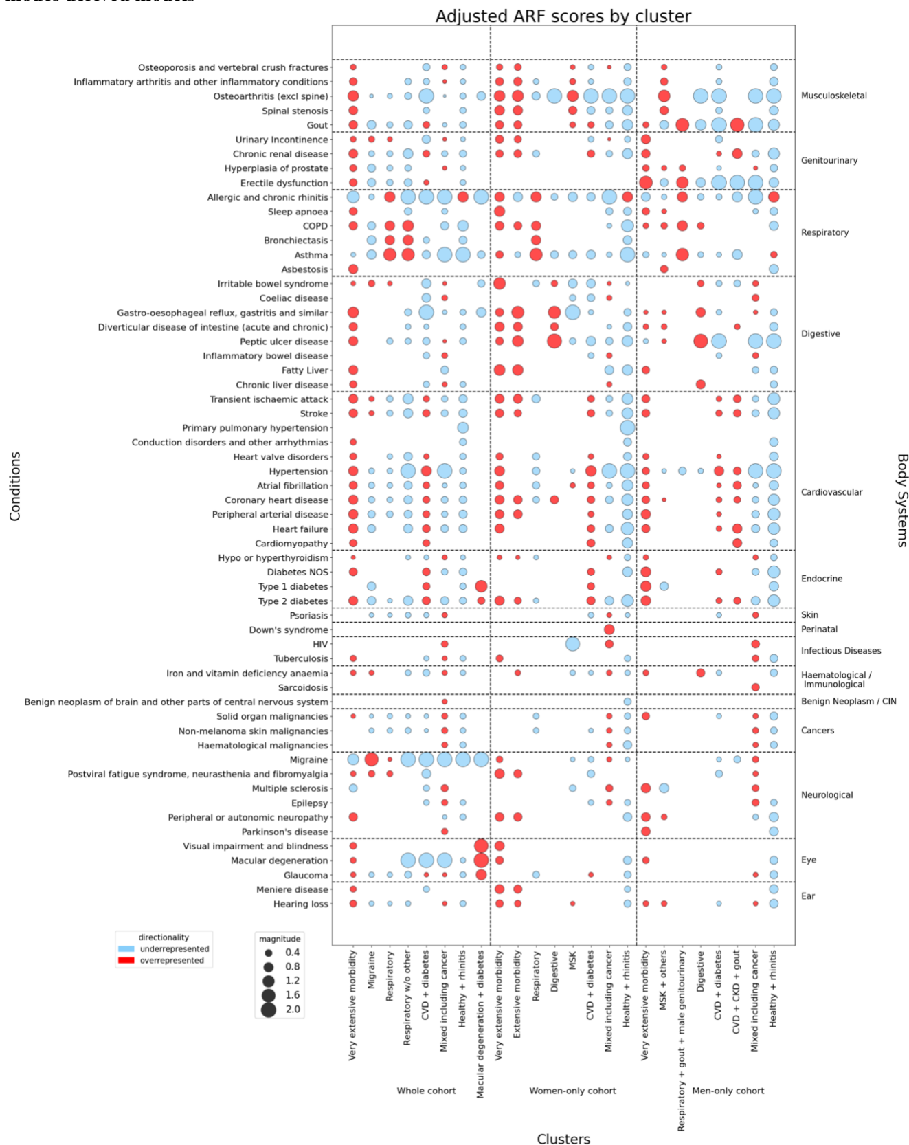
177 Fig. 1. Bubble heatmap shows under- and over-represented conditions in each cluster from the k - 178 modes derived models
