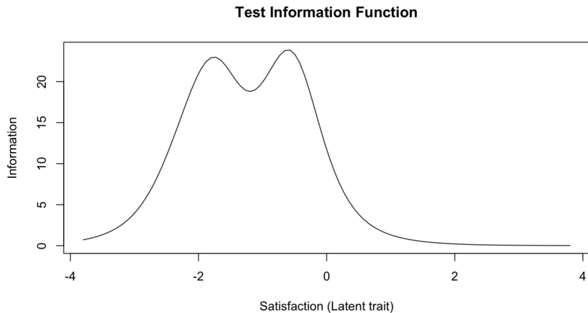
Figure 2. Test Information Function of the Experience of Service Questionnaire (unidimensional solution)
