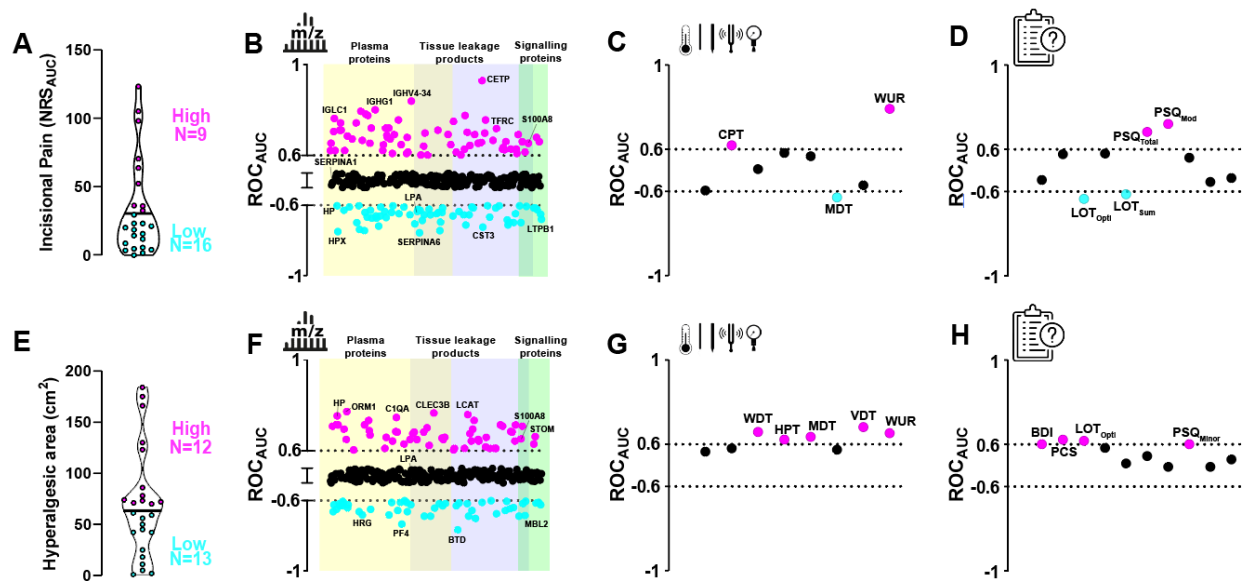
Fig. 3. Prognostic value of pre-incident blood plasma proteome profile, psychophysics, and psychosocial phenotype for post-incident outcome measures. (A) Volunteers were asked to judge the ongoing pain caused by the incision using the Numeric Rating Scale (NRS; 1-100). Integrated data from the first hour after the incision (first every minute for ten minutes, then every 5 minutes for 1h) were analyzed, and the areas under the curve (AUC) were plotted. Twenty-five volunteers (one volunteer was excluded because of technical reasons) were stratified into low (below the mean; N=16; cyan) or high (above the mean, N=9; magenta) responders depending on the rated pain perception within the acute post-incident phase (1 h post-injury). (B) Prognostic value of each of 311 pre-incident blood plasma proteins for high (magenta, AUC>0.6, 70 proteins) and low-responders (cyan, AUC<0.4, 72 proteins) for incisional pain. (C) Prognostic value of all parameters of psychophysical testing for high (magenta, AUC>0.6, CPT and WUR) and low-responders (cyan, AUC<0.4, MDT) for incisional pain. (D) Prognostic value of psychosocial questionnaires for high (magenta, AUC>0.6, PSQ-Total, PSQ-Moderate) and low-responders (cyan, AUC<0.4, LOT-Optimism, LOT-Summation) for incisional pain. (E) Upon incision injury, hyperalgesic area (HA) was assessed post 1 h (HA1) in 25 volunteers. Phenotyping was achieved by determining the total cohort's mean HA (68.65 cm 2 ). Volunteers with a lower HA1 were categorized as "low-responders" (N=13), and those with higher mean as "high-responders" (N=12). (F) Prognostic value of each of 311 pre-incident blood plasma proteins for high (magenta AUC>0.6, 60 proteins) and low-responders (cyan, AUC<0.4, 55 proteins) for hyperalgesic area 1h post-incident (HA1). (G) Prognostic value of all parameters of psychophysical testing for high (magenta, AUC>0.6, WDT, HPT, MDT, VDT, WUR) for HA1. (H) Prognostic value of psychosocial questionnaires for high (magenta, AUC>0.6, BDI, PCS, LOT-Optimism, and PSQ-Minor) for HA1. Abbreviations: CDT, cold detection threshold; CPT, cold pain threshold; HPT, heat pain threshold; MDT, mechanical detection threshold; MPS, mechanical pain sensitivity; MPT, mechanical pain threshold; PPT, pressure pain threshold; TSL, thermal sensory limen; VDT, vibration detection threshold; WDT, warmth detection threshold; WUR, wind-up ratio; BDI, Beck Depression Inventory; PCS, Pain Catastrophizing Scale; PSQ-Total, Perceived Stress Questionnaire-Total; PSQ-Moderate, Perceived Stress Questionnaire-Moderate; PSQ-Minor, Perceived Stress Questionnaire-Minor; LOT-Optimism, Life Orientation Test-Optimism; LOT-Pessimism, Life Orientation Test-Pessimism; LOT Summation, Life Orientation Test Summation; STAI x1, State-Trait Anxiety Inventory Form X1; STAI x2, State-Trait Anxiety Inventory Form X2.
