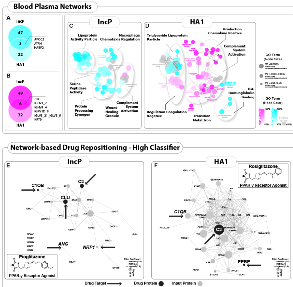
Fig. 5. Molecular mechanistic understanding and network-based drug repositioning analysis for pre-incipional biomarker signatures. (A) Pre-incipional protein classifier patterns for low-responders. A total of 47 unique proteins were identified for IncP and 22 for HA1 in low-responders, with an overlap of 3 proteins: APOC2, ATRN, and HABP2. (B) Pre-incipional protein classifier patterns for high-responders. A total of 49 unique proteins were identified for IncP and 32 for HA1 in high-responders, with an overlap of 6 proteins, specifically C8G, KRT9, and 7 different immunoglobulins. (C, D) The functional grouping of the enriched term-term interaction (TTI) network analysis, along with its associated proteins, was performed using ClueGO (v2.5.8), resulting in functional clusters (AutoAnnotate 1.3). (C) TTI-network analysis for IncP, highlighting terms exclusively present in high-responders, particularly clusters related to the innate immune system and the complement system via the classical and alternative pathways. (D) TTI-network analysis for HA1, emphasizing terms exclusively present in high-responders, with a focus on the complement system and innate immune response pathways. The data reveals significantly enriched GO terms, as indicated by P-values below 0.05, after applying the Benjamini-Hochberg correction. These terms are observed within a functionally grouped network, which accurately represents their interconnected relationships. Each node corresponds to a molecular function or process. Node colors are associated with phenotyping (high-responder in magenta shades; low-responder in cyan shades). Gray shades reflect unspecific terms which belong to both responder types. (E) Protein-protein-interaction (PPI) network drug repositioning results for IncP, showing the presence of the PPAR \gamma agonist Pioglitazone and its associated drug protein proteins (CLU, C3, C1QB), including ANG and NRP1 as input proteins. (F) PPI-network drug repositioning results for HA1, indicating the PPAR \gamma agonist Rosiglitazone and its associated drug proteins (C3, PPBP), with C1QB also identified as an input protein.
