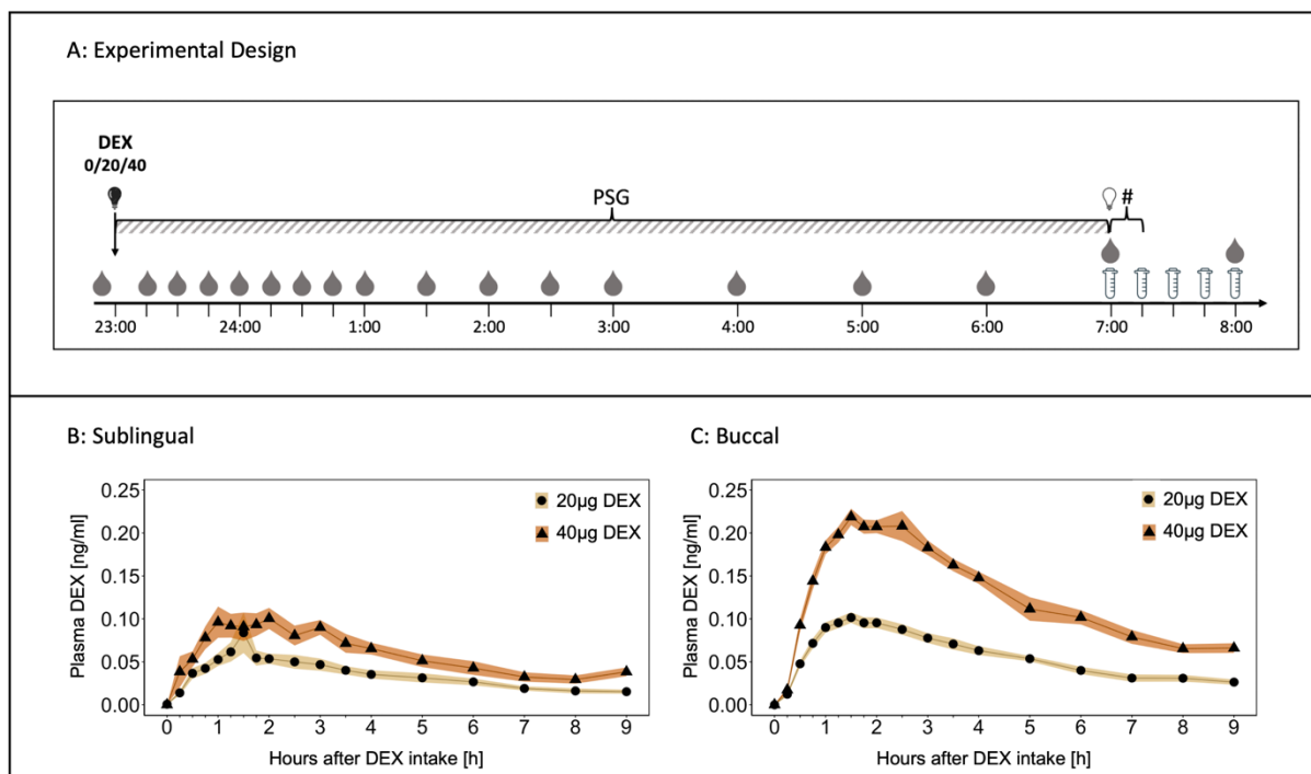
Figure 1: Experimental design and pharmacokinetic profiles of dexmedetomidine (DEX) after sublingual and buccal oro-dispersible tablet (ODT) intake. (A) Time points of blood draws (●), saliva sampling (🧴), and post-awakening testing (#) are indicated. The study drugs (0/20/40 µg DEX) were administered at 23:00 when lights were switched off (💡) and the polysomnographic recording was initiated (time point '0'). The participants were awoken and lights were turned on at 07:00 (time point '8'). (B) Evolution of DEX plasma concentration after intake of sublingual ODT. (C) Evolution of DEX plasma concentration after intake of buccal ODT. Yellow lines connecting black dots: 20 µg DEX intake at bedtime. Orange lines connecting black triangles: 40 µg DEX intake at bedtime. Yellow/orange shadings indicate standard errors of the means.
