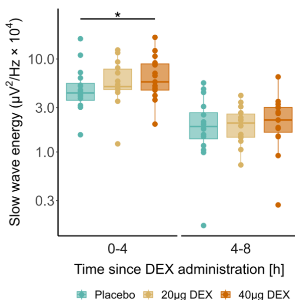
Figure 3. The EEG slow wave energy in the 0.75-4.0 Hz range in NREM sleep stages N2 & N3 was quantified in the first (0-4 h after intake) and second (4-8 h after intake) halves of the nights following buccal ODT administration at bedtime. Box plots: horizontal lines mark the median, lower and upper hinges that correspond to the 25 th and 75 th percentiles, whiskers extend to the last value within 1.5x of the interquartile range, and outliers are individually plotted. Blue: placebo; yellow: 20 \mu\text{g} DEX; orange: 40 \mu\text{g} DEX. Note that the values are presented on a logarithmic scale. The asterisk indicates the significant difference between the 40 \mu\text{g} DEX and placebo conditions in the first half of the experimental nights.
