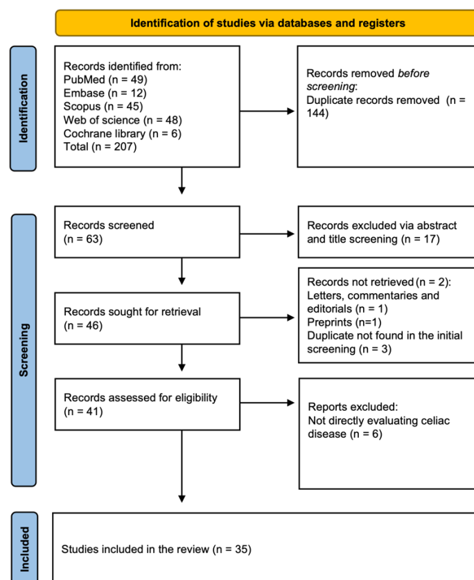
Figure 1: PRISMA flowchart.
