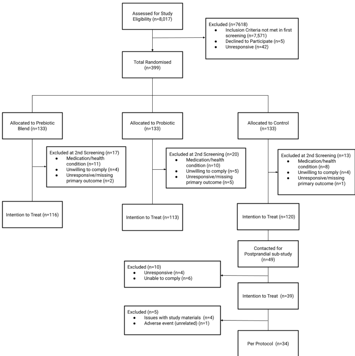
Figure 2. CONSORT Diagram
