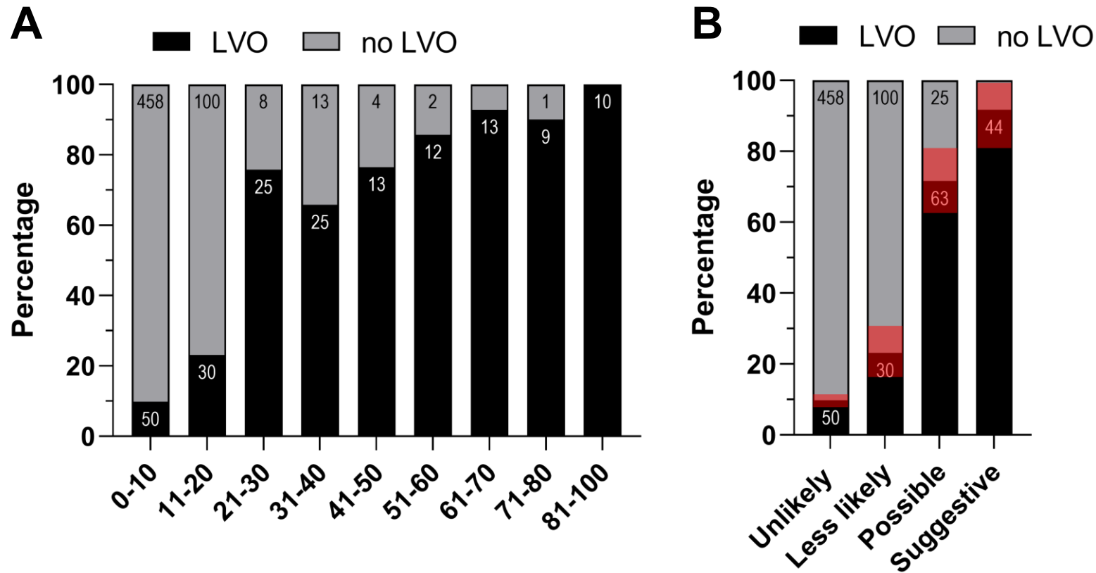
Figure 4. (A) Observed frequency of large vessel occlusion (LVO) across deciles of JLK-CTL LVO scores. Numbers within bars indicate the patient count. (B) Observed frequency of LVO across groups categorized as unlikely (LVO score 0–10), less likely (11–20), possible (21–50), and suggestive (50–100) based on observed frequencies of LVO. Red boxes represent the 95% confidence intervals for the observed frequency of LVO.
