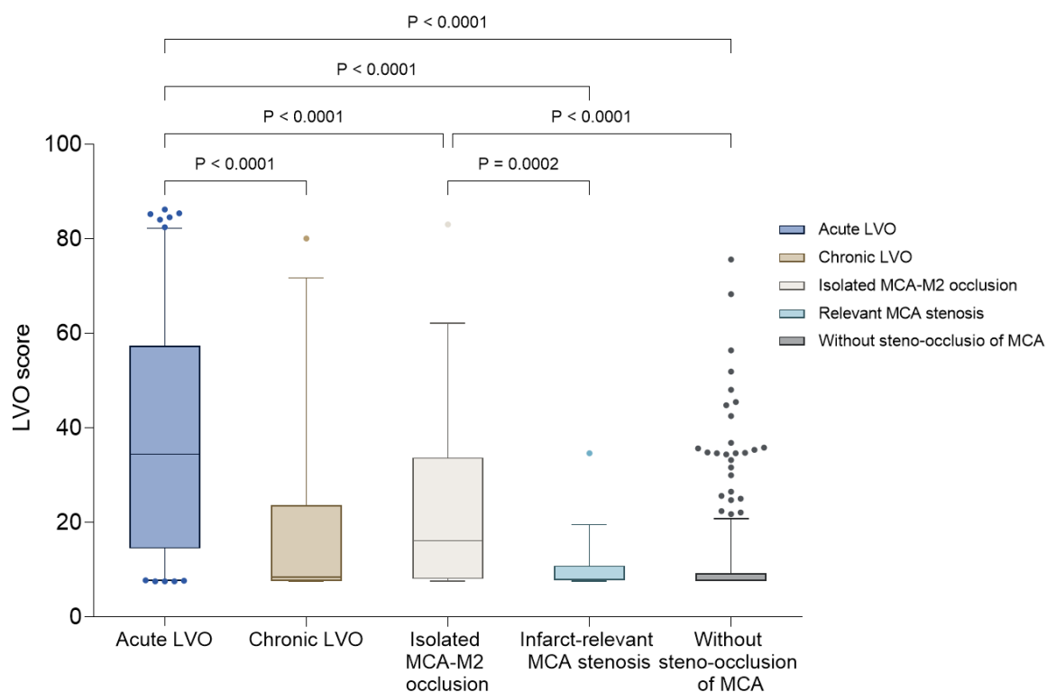
Figure 2. Box plots illustrating JLK-CTL LVO scores across subgroups categorized by steno-occlusion of the middle cerebral artery (MCA). Statistical comparisons were conducted using ANOVA followed by Tukey post-hoc analysis. LVO=large vessel occlusion.
