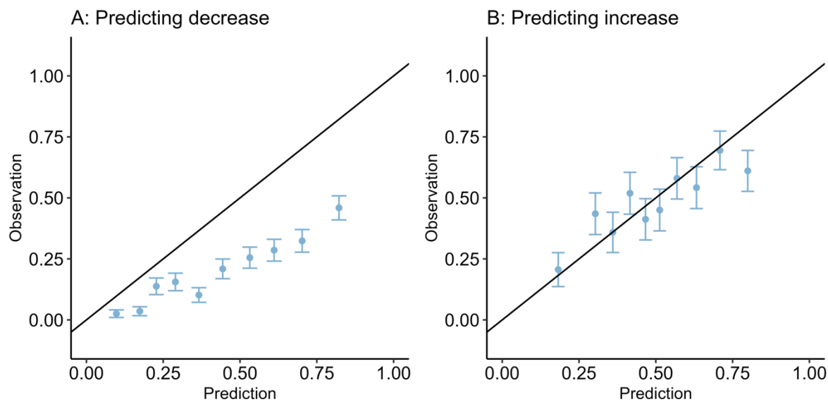
Figure 2 Calibration plots
