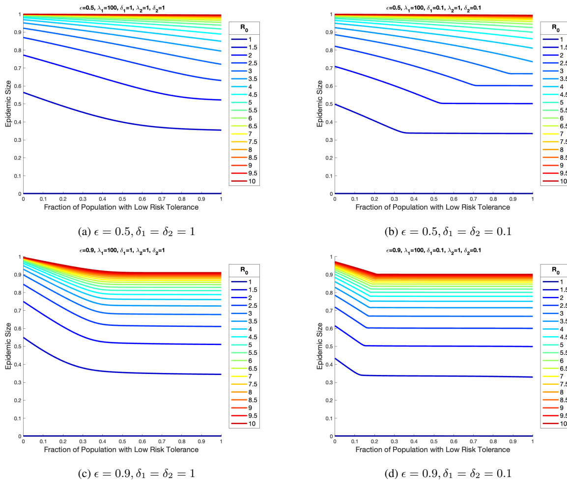
Figure 4: Final epidemic size versus fraction of population that are risk-averse ( S_1 ). Simulations in the left column have a higher \delta than simulations in the right column. The other simulation parameters and initial conditions are \lambda_1 = 100, \lambda_2 = 1, I = 10^{-7}, P_1 = P_2 = 0, R = 0 .
