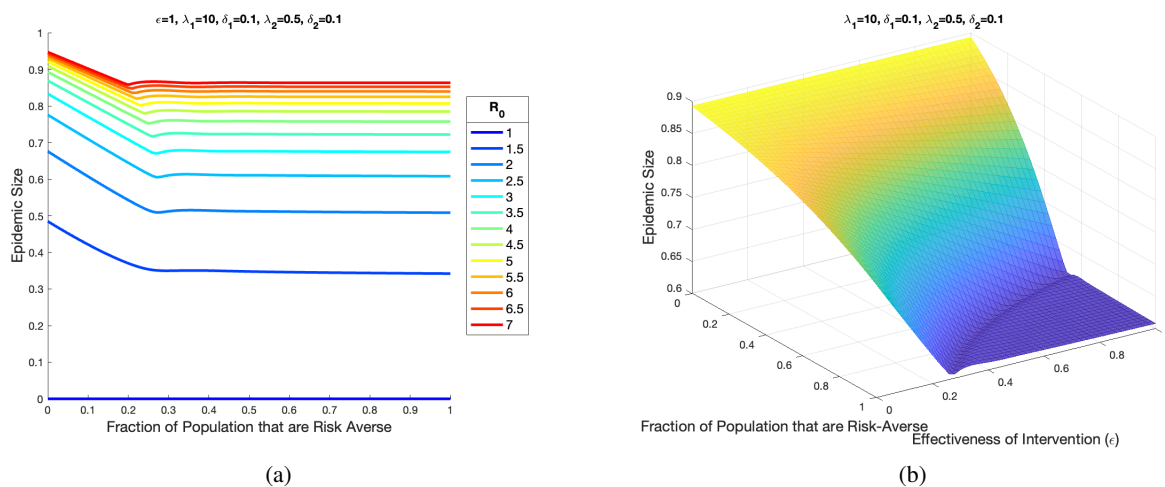
Figure 6: (a) Final epidemic size as a function of the proportion of the population that are risk averse ( S_1 ). Model parameters and initial conditions for the simulation are \epsilon = 1, \lambda_1 = 10, \lambda_2 = 0.5, \delta_1 = 0.1, \delta_2 = 0.1, I(0) = 10^{-7}, x_{S_2}(0) = 1 - x_{S_1} - I(0), P_1(0) = P_2(0) = 0, R(0) = 0 . (b) Same as in (a) except now the effectiveness of the intervention ( \epsilon ) is allowed to vary.
