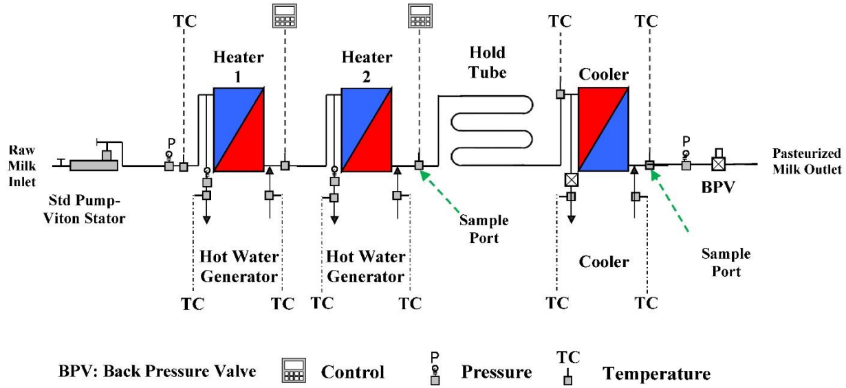
Figure1. Schematic of the HTST continuous flow pasteurizer with inline sampling ports.
