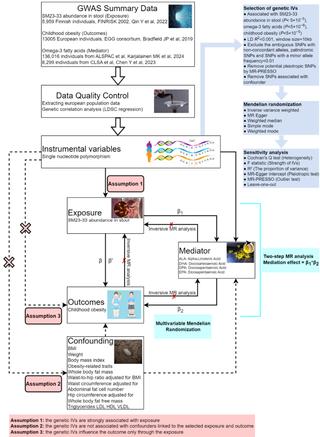
Figure 1. Overall study design plan. GWAS, genome-wide association studies; SNPs: single-nucleotide polymorphisms; \beta : the total causal effects of exposure on outcome was
