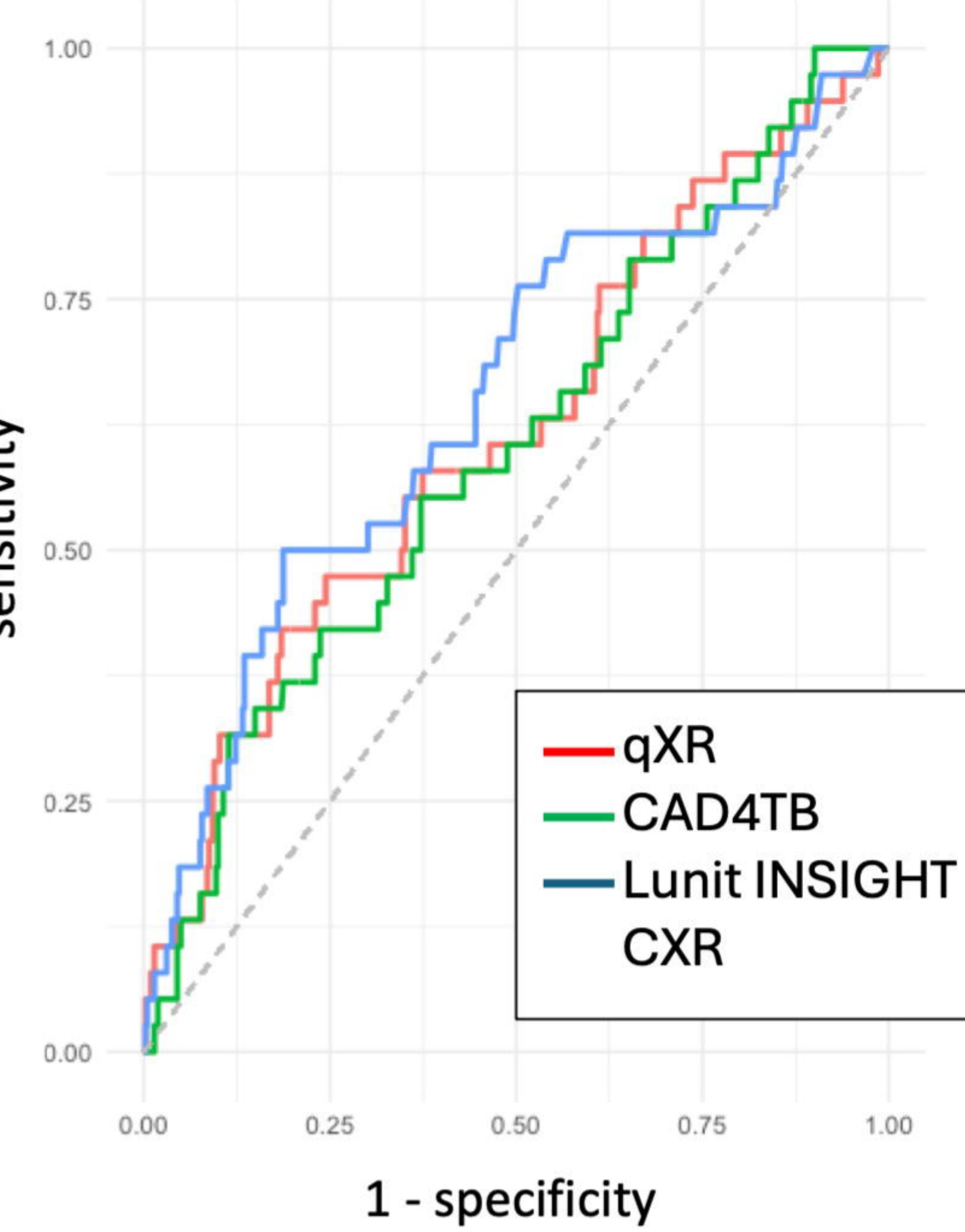
AUC ROC: Incident TB
