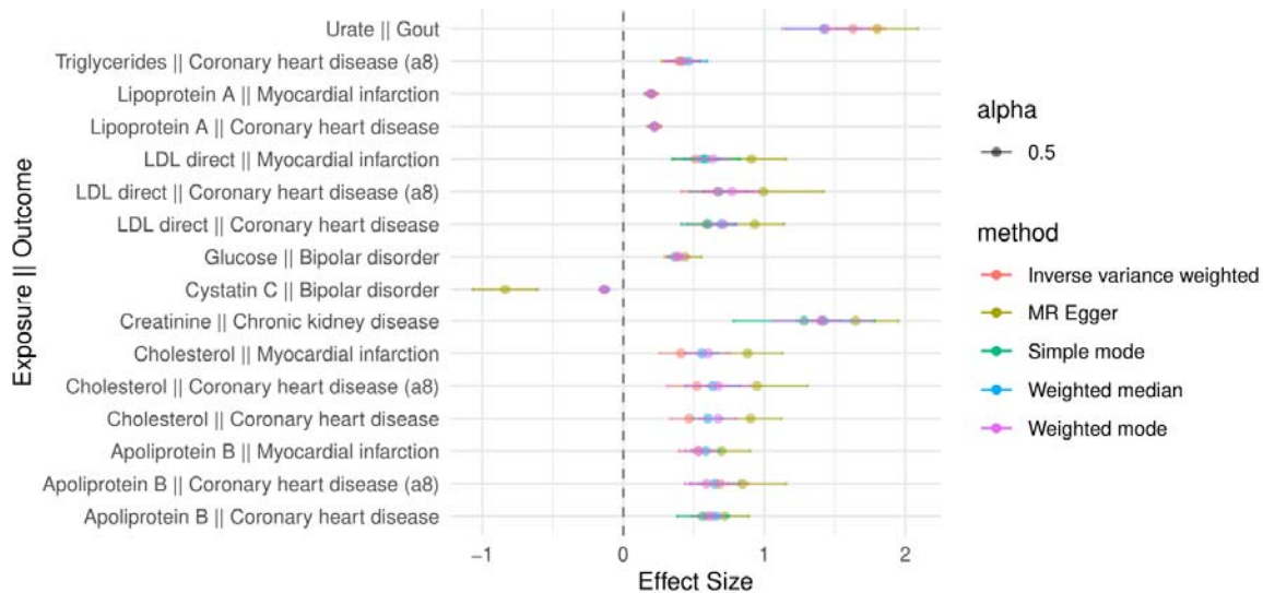
Figure 2. Forest Plot of Mendelian Randomization Analysis Results Assessing the Causal Effects of Circulating Biomarkers on Diseases. The forest plot illustrates the estimated causal effects of top-16 significantly associated (Bonferroni p-value < 0.05) biomarkers on the risk of various diseases based on Mendelian randomization (MR) analysis consistent across 4 or more methods. Each row represents a different MR association, with the biomarker as the exposure and the disease as the outcome. The points represent different effect size estimates from different MR methods and the 95% confidence intervals (based on standard errors of the effect size estimates) are displayed by the horizontal lines forming around the average effect sizes of different methods.
