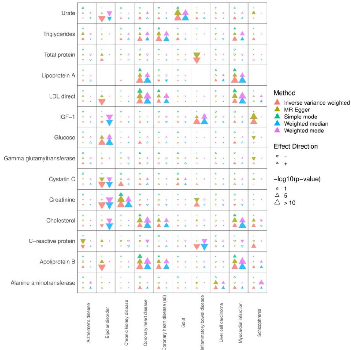
Figure 1. Heatmap summarizing the key findings of this study, including the most significant findings from the MR Egger analysis. MR analyses were conducted using 5 methods: Inverse variance weighted, MR Egger, Simple mode, Weighted Median, and Weighted Mode. Larger arrow sizes correspond to more significant results and the directionality of the arrow indicates a posi-
