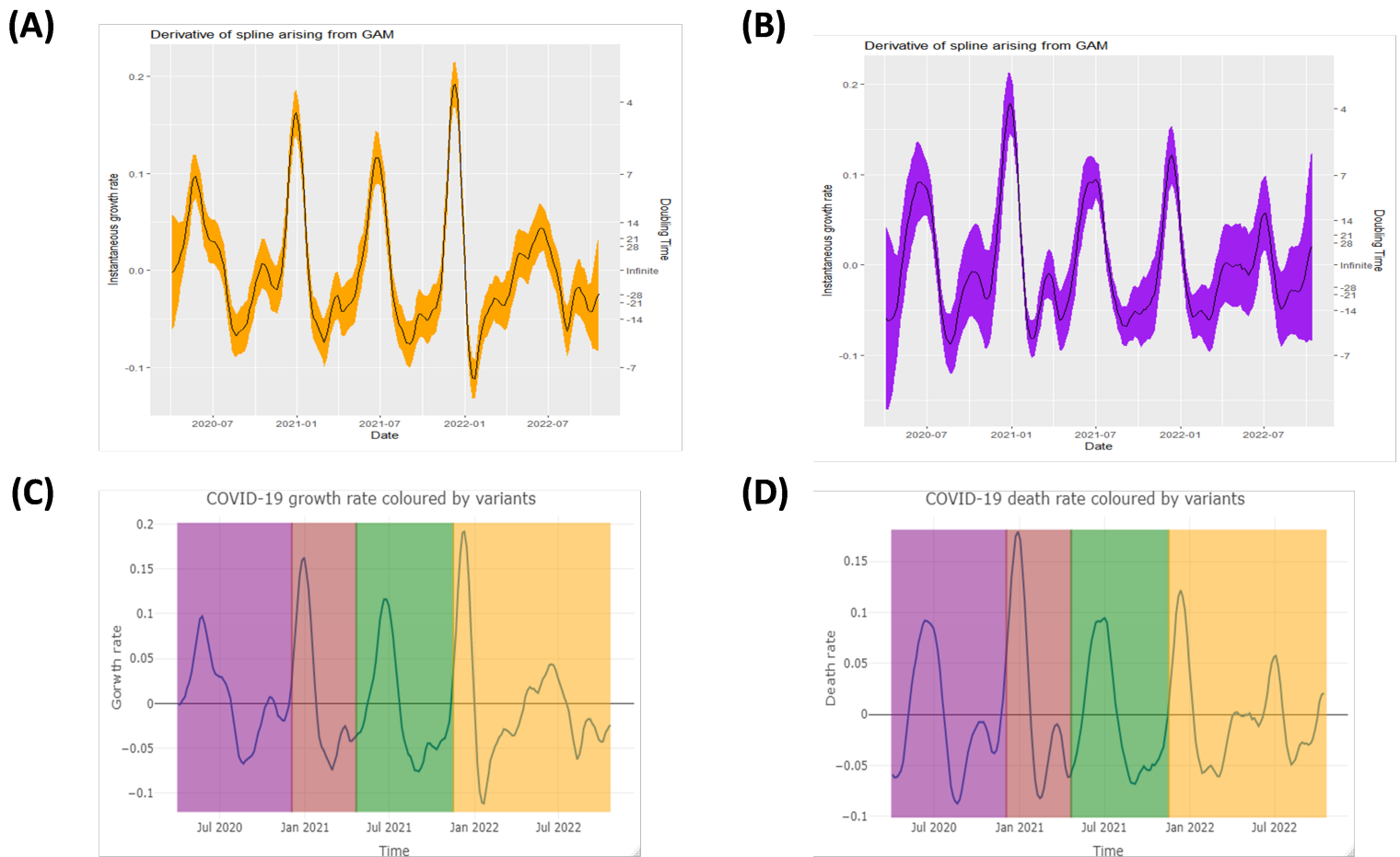
Figure 3: Growth rate and doubling time. (A) Growth rate and doubling time curve for cases. (B) Growth rate and doubling time curve for deaths. (C) Growth rate for cases: Other (purple), Beta (brown), Delta (green) and Omicron (orange). (D) Growth rate for deaths: Other (purple), Beta (brown), Delta (green) and Omicron (orange).
