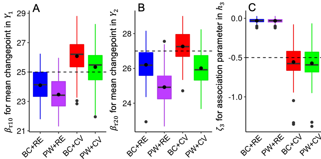
Figure 8. Distributions of posterior means for main changepoint and association parameters in Scenario 4 (community cohort with current value association structure). Panels A, B, and C represent the distributions of estimated posterior means for \beta_{1\tau_0} (the mean changepoint parameter in Y_1 ), \beta_{2\tau_0} (the mean changepoint parameter in Y_2 ), and \zeta_3 (the association parameter between longitudinal and survival processes in h_3 ), respectively. In each panel, the boxes denote the posterior means across all simulated datasets based on each method, while the dashed line indicates the true value for the parameter. PW: piecewise model; BC: bent-cable model; RE: shared random effect structure; CV: current value structure.
