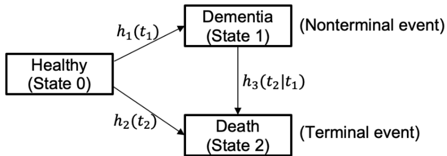
Figure 2. Three health states with semi-competing risks. h_1(t_1) is the hazard function for dementia at time t_1 , h_2(t_2) is the hazard function for death at time t_2 , and h_3(t_2|t_1) denotes the hazard function for death at time t_2 given that the participant develop dementia at time t_1 .
