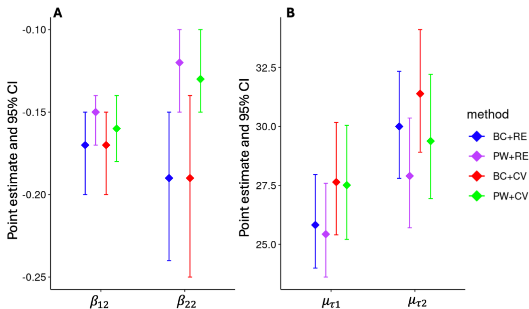
Figure 10. Comparison of estimates for slope differences after the changepoint and mean changepoint location. In Panel A, the bars denote the posterior means and its 95% credible intervals for slope differences after the changepoint based on each method. \beta_{12} and \beta_{22} in the x-axis denote slope differences after the changepoint in memory and language cognitive domains, respectively. In Panel B, the bars denote the posterior means and its 95% credible intervals for estimated mean changepoints based on each method. \mu_{\tau 1} and \mu_{\tau 2} in the x-axis denote estimated mean changepoints in memory and language cognitive domains, respectively. PW: piecewise model; BC: bent-cable model; RE: shared random effect structure; CV: current value structure. CI: credible interval.
