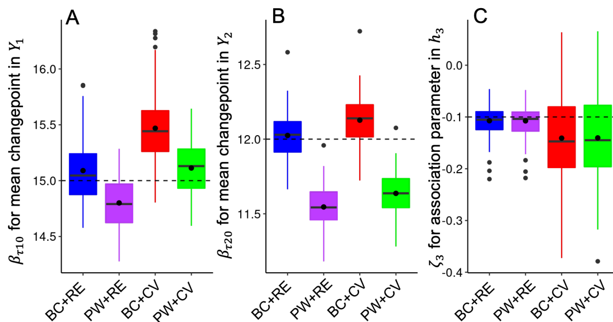
Figure 5. Distributions of posterior means for main changepoint and association parameters in Scenario 1 (disease cohort with shared random effect association structure). Panels A, B, and C represent the distributions of estimated posterior means for \beta_{1\tau_0} (the mean changepoint parameter in Y_1 ), \beta_{2\tau_0} (the mean changepoint parameter in Y_2 ), and \zeta_3 (the association parameter between longitudinal and survival processes in h_3 ), respectively. In each panel, the boxes denote the posterior means across all simulated datasets based on each method, while the dashed line indicates the true value for the parameter. PW: piecewise model; BC: benticable model; RE: shared random effect structure; CV: current value structure.
