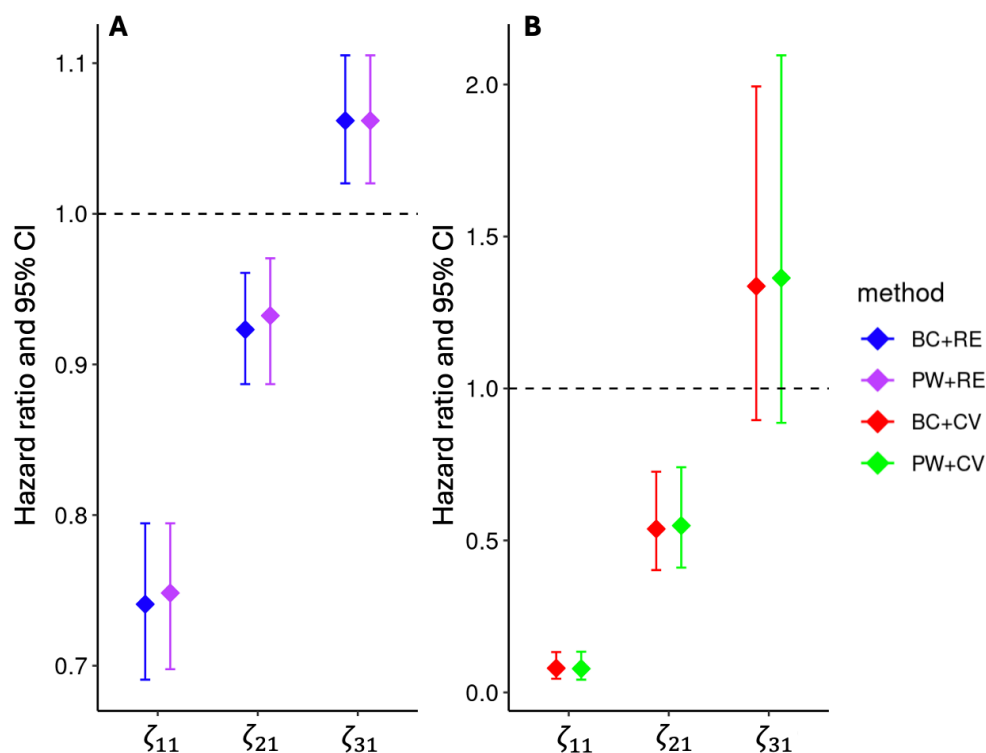
Figure 11. Comparison of estimates for association parameters linking the longitudinal and survival processes. In Panel A, the bars denote the posterior means and its 95% credible intervals for the association parameters between the changepoint in the longitudinal process and the survival process based on each method. \zeta_{11} , \zeta_{11} , and \zeta_{31} in the x-axis denote the association parameters in h_1 , h_2 , and h_3 , respectively. In Panel B, the bars denote the posterior means and its 95% credible intervals for the association parameters between the true unobserved value of the longitudinal cognitive measures and the survival process based on each method. \zeta_{11} , \zeta_{11} , and \zeta_{31} in the x-axis denote the association parameters in h_1 , h_2 , and h_3 , respectively. PW: piecewise model; BC: bent-cable model; RE: shared random effect structure; CV: current value structure. CI: credible interval.
