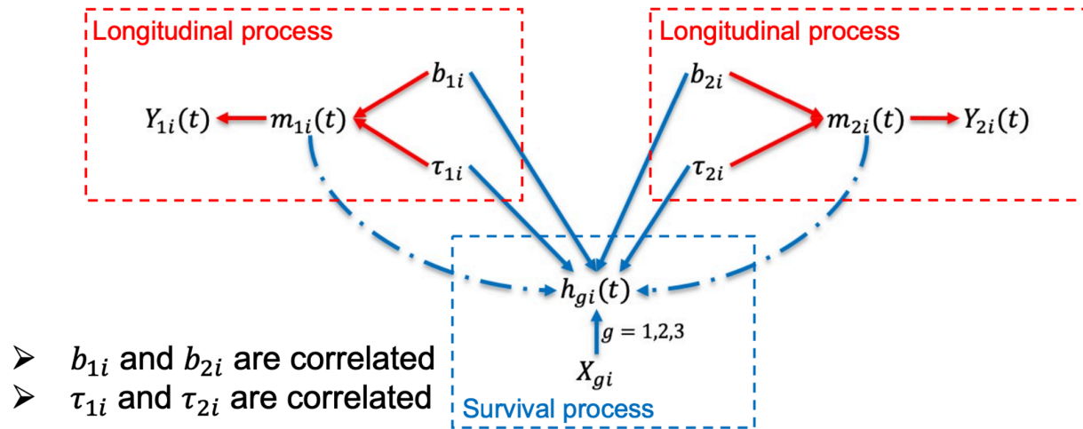
Figure 3. The joint model framework. Two red boxes represent the longitudinal process for two longitudinal measures, and the blue box is the survival process. Y_{1i} and Y_{2i} are two longitudinal measures, m_{1i}(t) and m_{2i}(t) are the true unobserved values for two longitudinal measures, \tau_{1i} and \tau_{2i} are two changepoints, b_{1i} and b_{2i} are random intercepts and slopes for the first and second longitudinal measures. h_{gi}(t) denotes the hazard function for each health state transition, and X_g is a baseline covariate associated with each hazard function. Both longitudinal and survival processes are linked by either random effects (solid blue lines for the shared random effect model) or the true unobserved values of longitudinal measures (dashed blue lines for the current value model).
