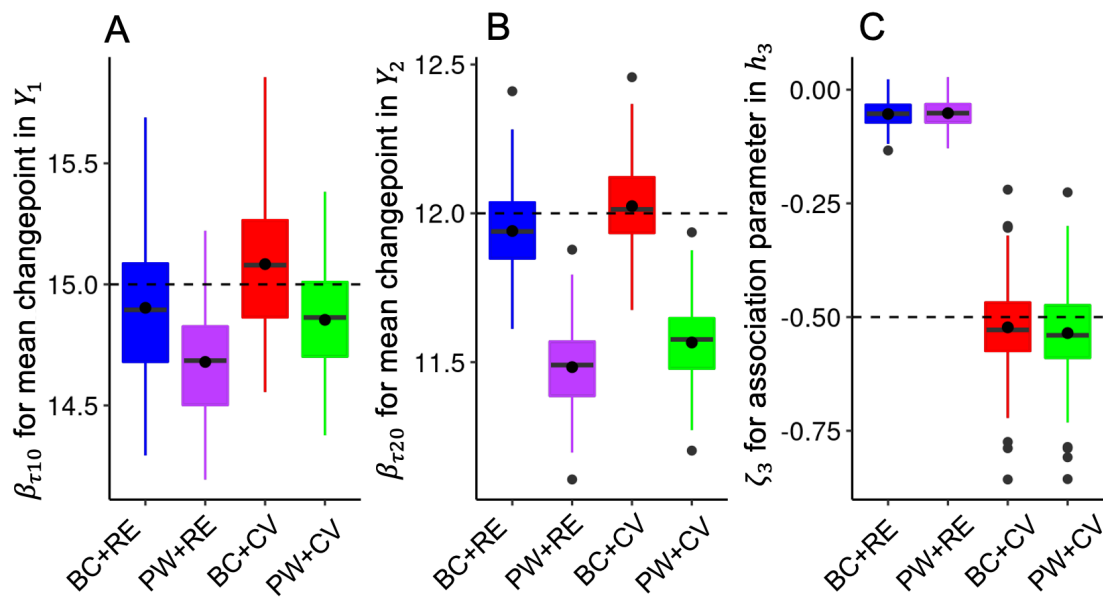
Figure 6. Distributions of posterior means for main changepoint and association parameters in Scenario 2 (disease cohort with current value association structure). Panels A, B, and C represent the distributions of estimated posterior means for \beta_{1\tau_0} (the mean changepoint parameter in Y_1 ), \beta_{2\tau_0} (the mean changepoint parameter in Y_2 ), and \zeta_3 (the association parameter between longitudinal and survival processes in h_3 ), respectively. In each panel, the boxes denote the posterior means across all simulated datasets based on each method, while the dashed line indicates the true value for the parameter. PW: piecewise model; BC: bent-cable model; RE: shared random effect structure; CV: current value structure.
