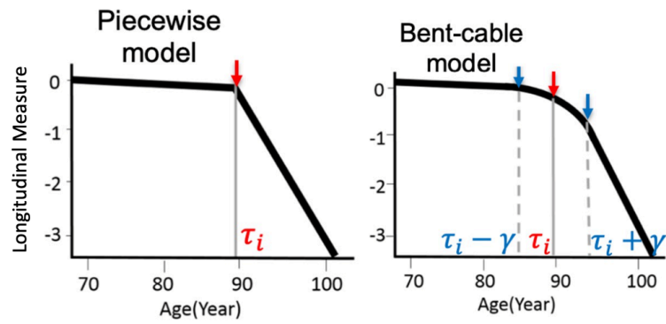
Figure 1. The visualization of the piecewise model (left) and the Bent-Cable model (right). The y-axis represents the value of a longitudinal measure, and the x-axis represents age. \tau_i is the changepoint for participant i . [\tau_i - \gamma, \tau_i + \gamma] denotes the smooth transition zone for the Bent-Cable model.
