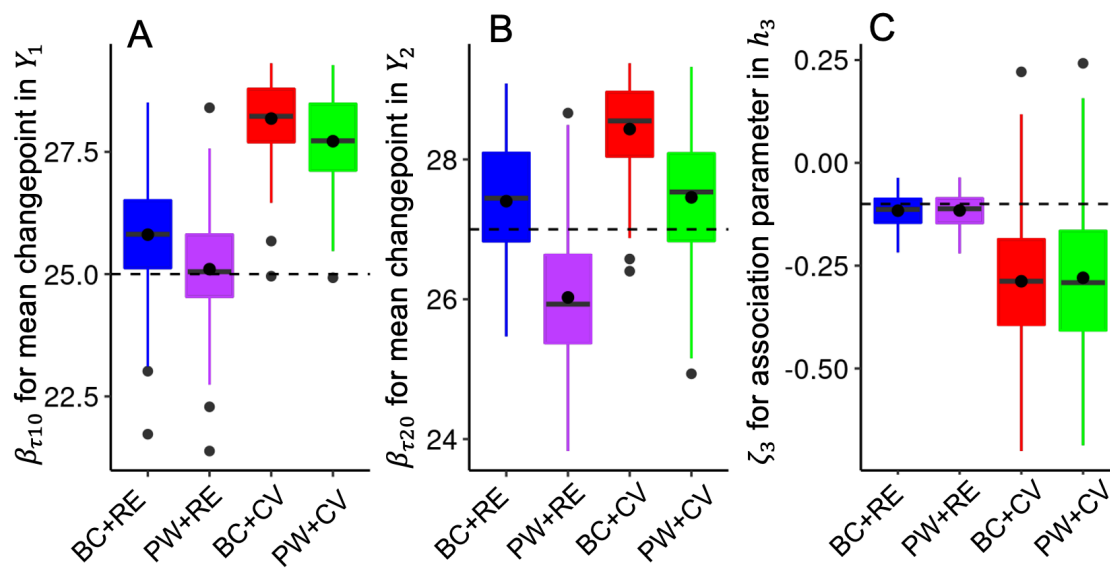
Figure 7. Distributions of posterior means for main changepoint and association parameters in Scenario 3 (community cohort with shared random effect association structure). Panels A, B, and C represent the distributions of estimated posterior means for \beta_{1\tau_0} (the mean changepoint parameter in Y_1 ), \beta_{2\tau_0} (the mean changepoint parameter in Y_2 ), and \zeta_3 (the association parameter between longitudinal and survival processes in h_3 ), respectively. In each panel, the boxes denote the posterior means across all simulated datasets based on each method, while the dashed line indicates the true value for the parameter. PW: piecewise model; BC: bent-cable model; RE: shared random effect structure; CV: current value structure.
