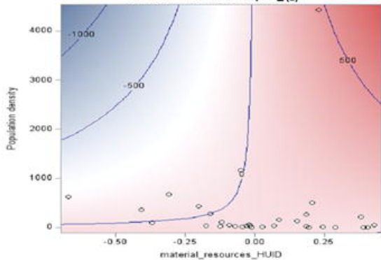
Contour Fit Plot for Mpox_(c)
