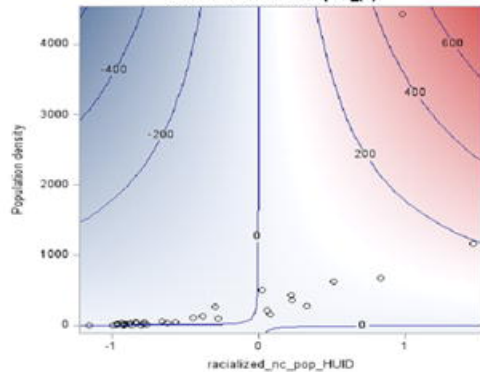
Contour Fit Plot for Mpox_(c)
