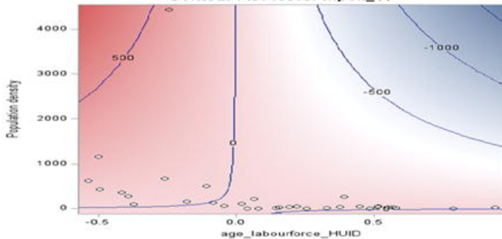
Contour Fit Plot for Mpox_(c)
