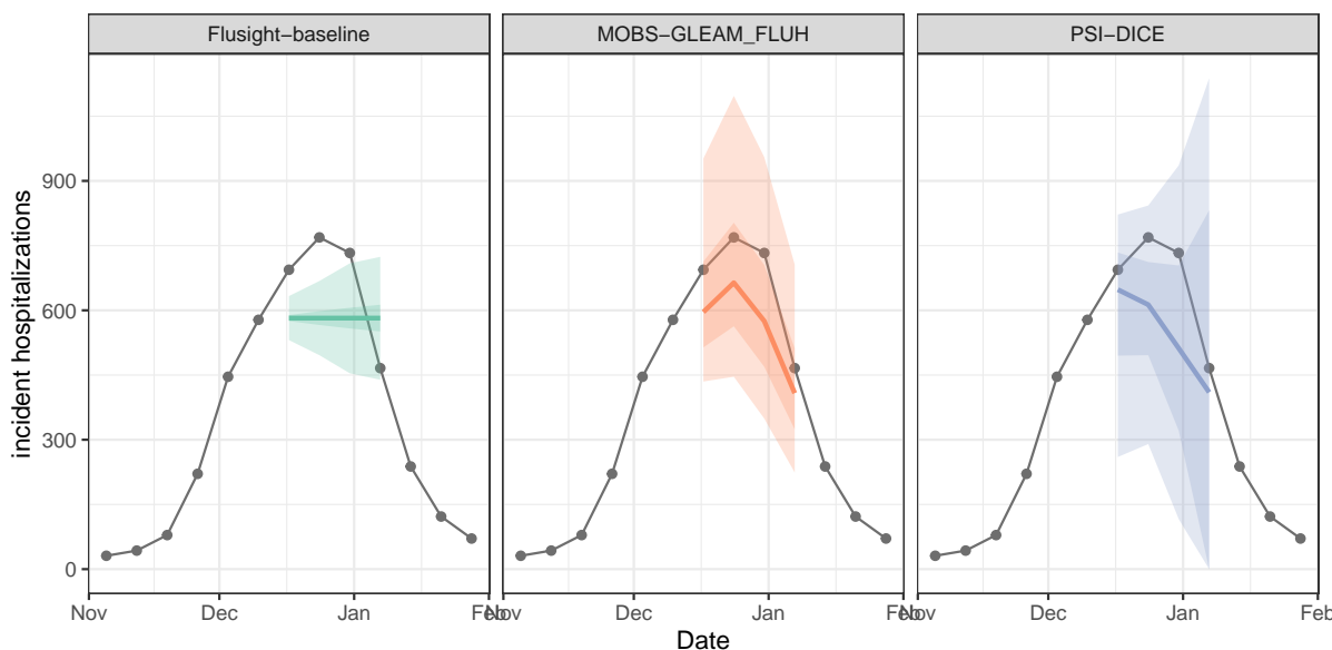
Figure 2: One example set of quantile forecasts of weekly incident influenza hospitalizations in Massachusetts from each of three models (panels). Forecasts are represented by a median (line), 50% and 90% prediction intervals (ribbons). Gray points represent observed incident hospitalizations.
