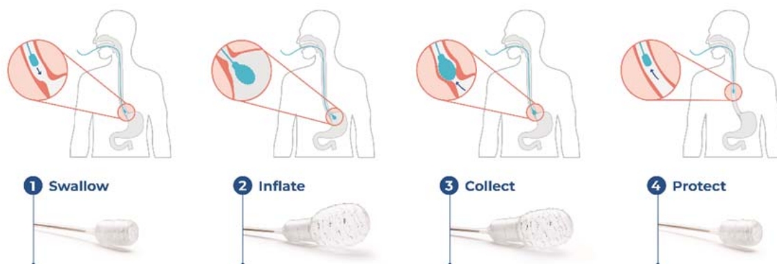
Figure 1. EsoCheck cell collection process
