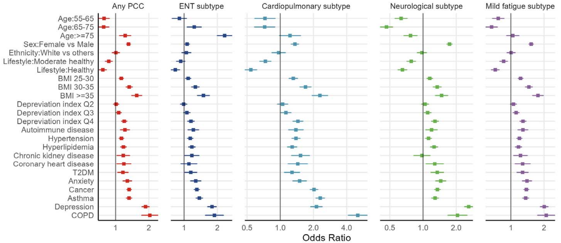
Figure 3. Associations of host-related factors with PCC and its subtypes
