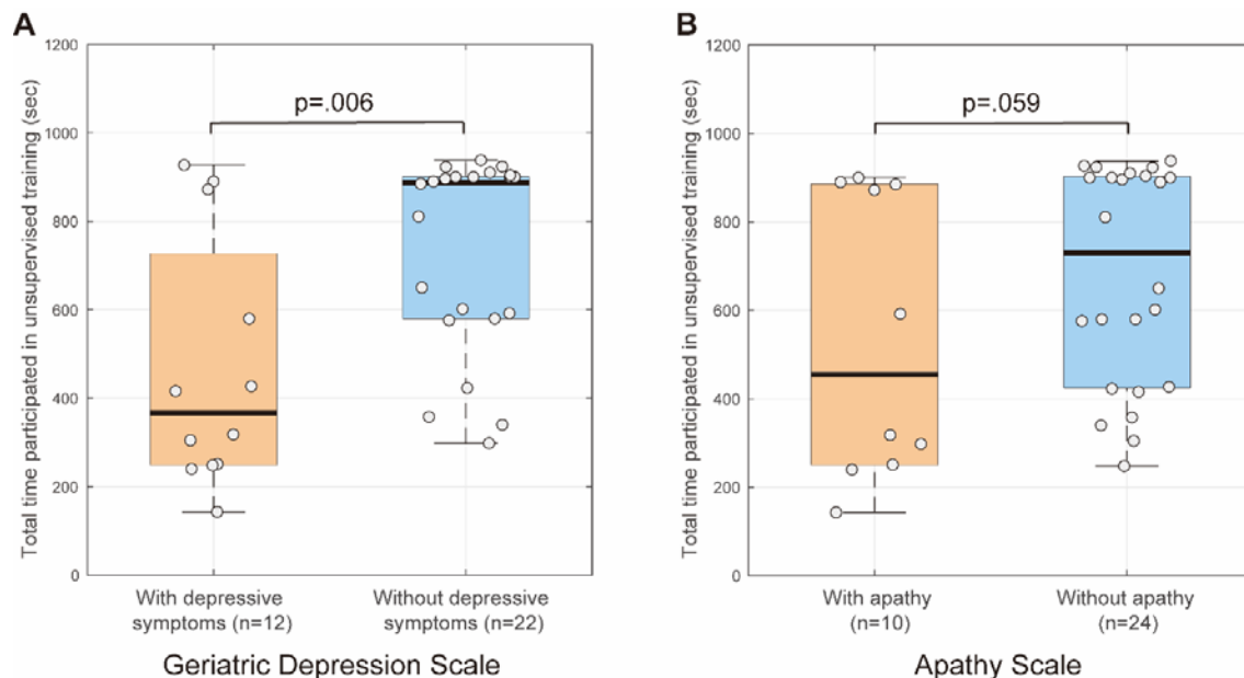
Figure 1. Comparisons of the total time spent in unsupervised training (A) between the groups with and without depressive symptoms and (B) between the groups with and without apathy. Data are presented as median (bold black line) and interquartile range with individual plot (grey circle).
