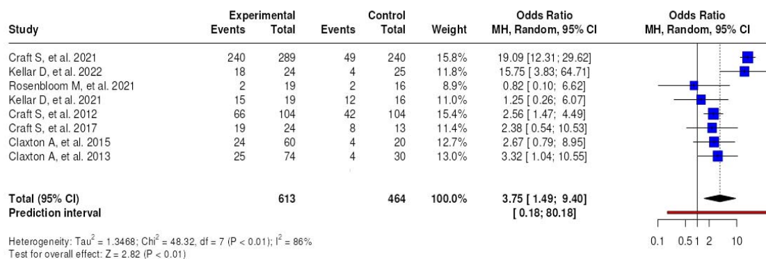
Figure 4. Comparative assessment of intranasal insulin (INI) versus placebo on global cognitive function in the overall study population
