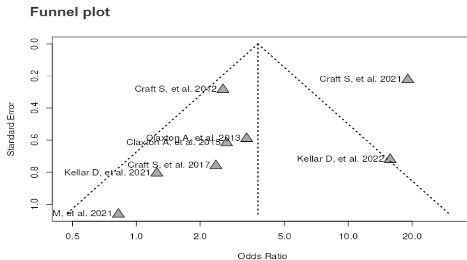
Figure 5. Funnel plot for meta-analysis
