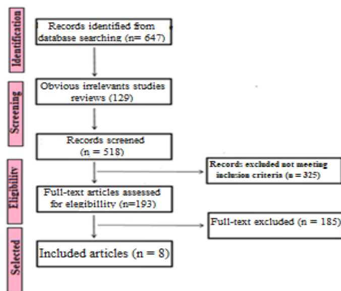
Figure 1. Flowchart of the selection process for the 8 studies included.
