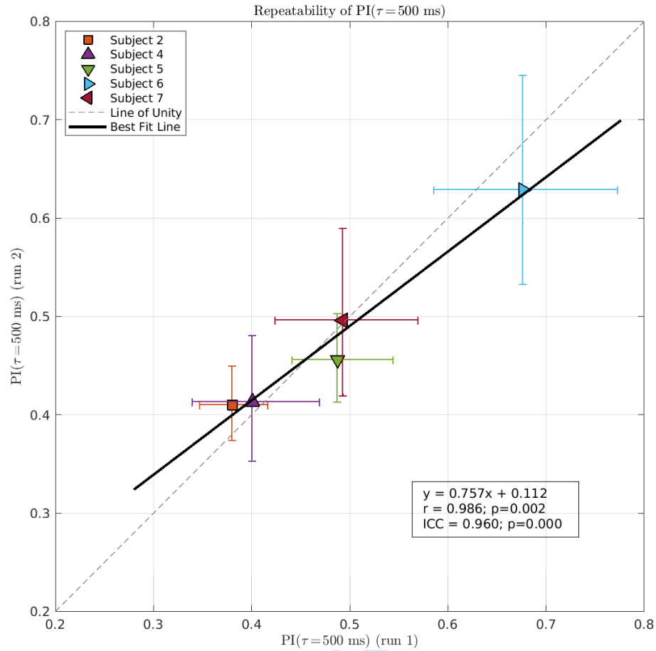
Figure 6: Repeatability of PI( \tau=500 ms) across subjects. The x-axis denotes the PI of run 1, and the y-axis denotes the PI of run 2. The data points are the measured values from the 5 subjects with repeats of the \tau = 500 ms scan. The error bars indicate the 95% confidence intervals of the values. The values follow the line of unity closely, indicating excellent test-repeat repeatability. This is further supported by the high Pearson correlation coefficient r = 0.986 ( p = 0.002 ) and ICC = 0.960 ( p < 0.001 ).
