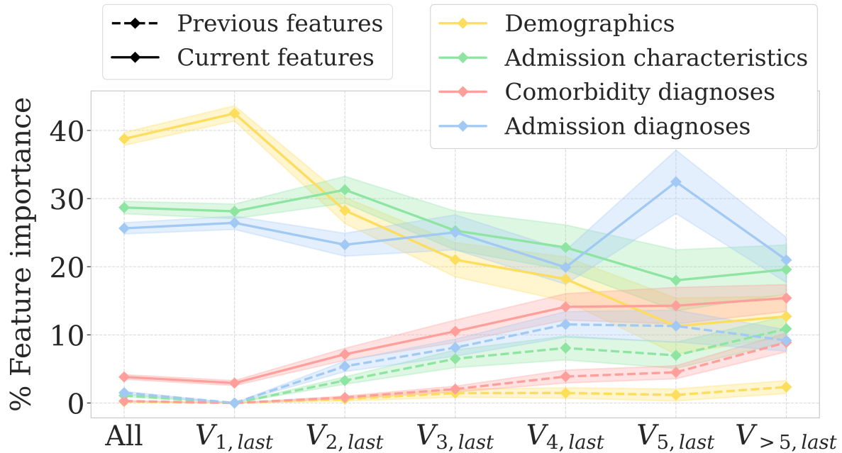
Fig. 5 Post-hoc analyses of feature importance of the final ELSTM trained with AdmDemoDx predictors. Importance of each feature is computed using feature permutation [26] over 100 bootstraps. Shaded regions indicate variations within one standard deviation of the mean over 100 bootstraps. Importance of previous features increases as the size of patients' history gets longer
