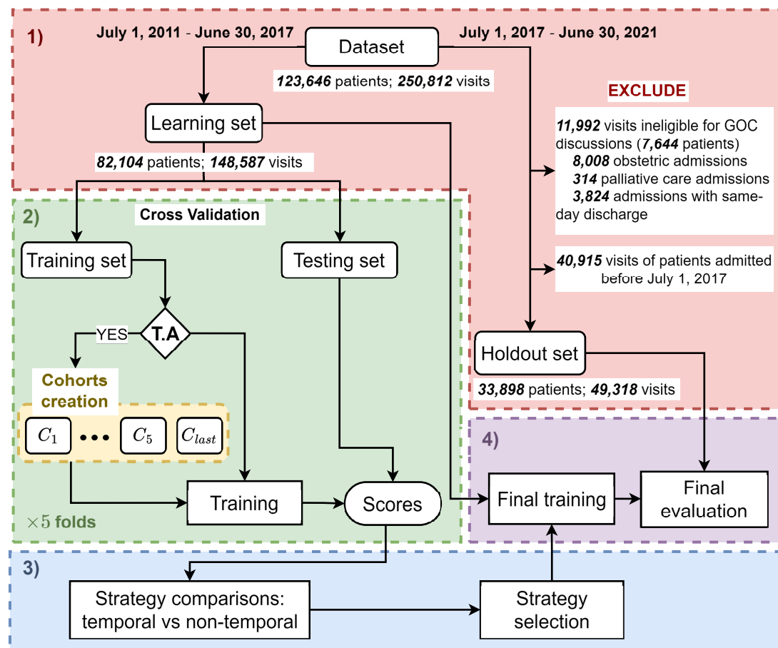
Fig. 2 Experimental setup for model comparisons and final evaluation. 1) Temporal division of the dataset into a learning set and a holdout set . 2) Evaluation of the predictive performance of each model on 5 testing sets using a 5-fold cross-validation over the patients of the learning set. The same data splits are used for all models. Baseline models (RF, BLSTM) are trained on all the visits, while each temporal model LSTM k comprising the ELSTM is trained using a temporal cohort C_k . The scores are reported on specific patients of the testing sets . The training of each model includes the optimization of hyperparameters, except for the temporal models, for which we only optimize the hyperparameters of LSTM last . Details on hyperparameter optimization are shown in Appendix A. 3) Comparison of the temporal and non-temporal strategy and selection of the best strategy based on performance. The latter is measured using the mean and standard deviation of the scores on the 5 testing sets. 4) Final evaluation of the selected strategy on the holdout set. The final model predictions are then compared to usual care to quantify clinical utility
