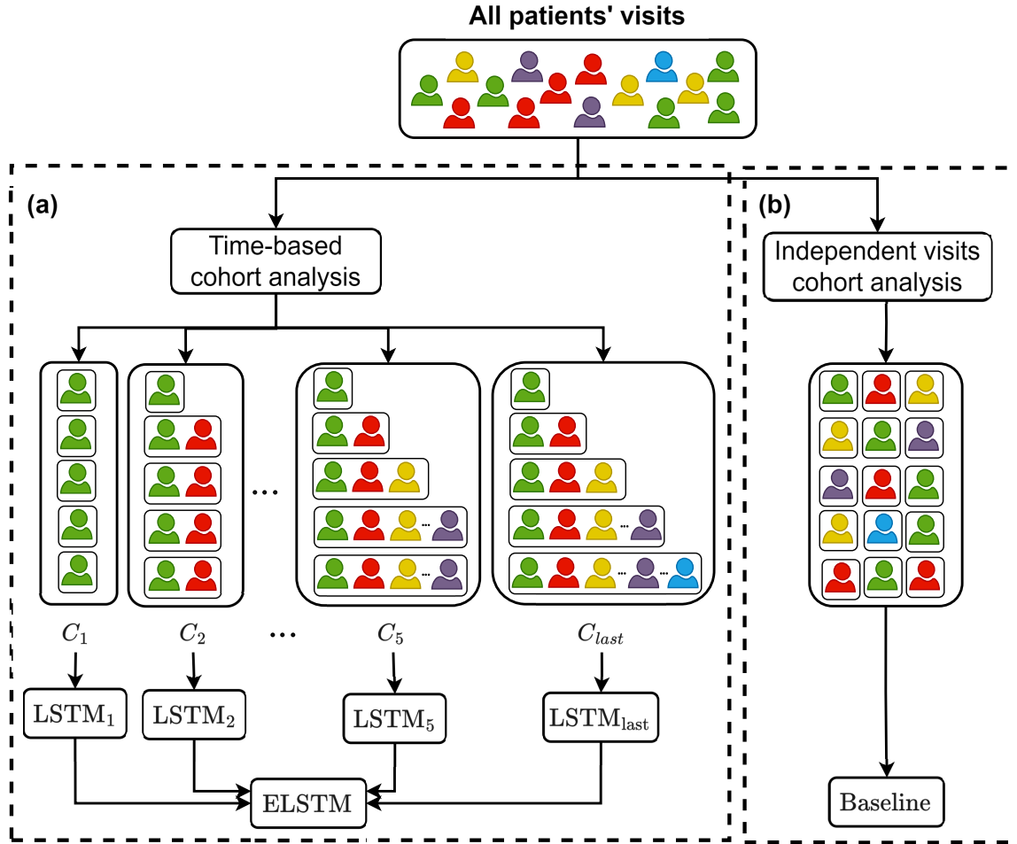
Fig. 1 Study overview. (a) The ELSTM averages predictions of multiple LSTMs trained using different cohorts of the same patients. Each cohort includes the patient’s history up to a specific visit. (b) Baseline models consider patients visits independently
