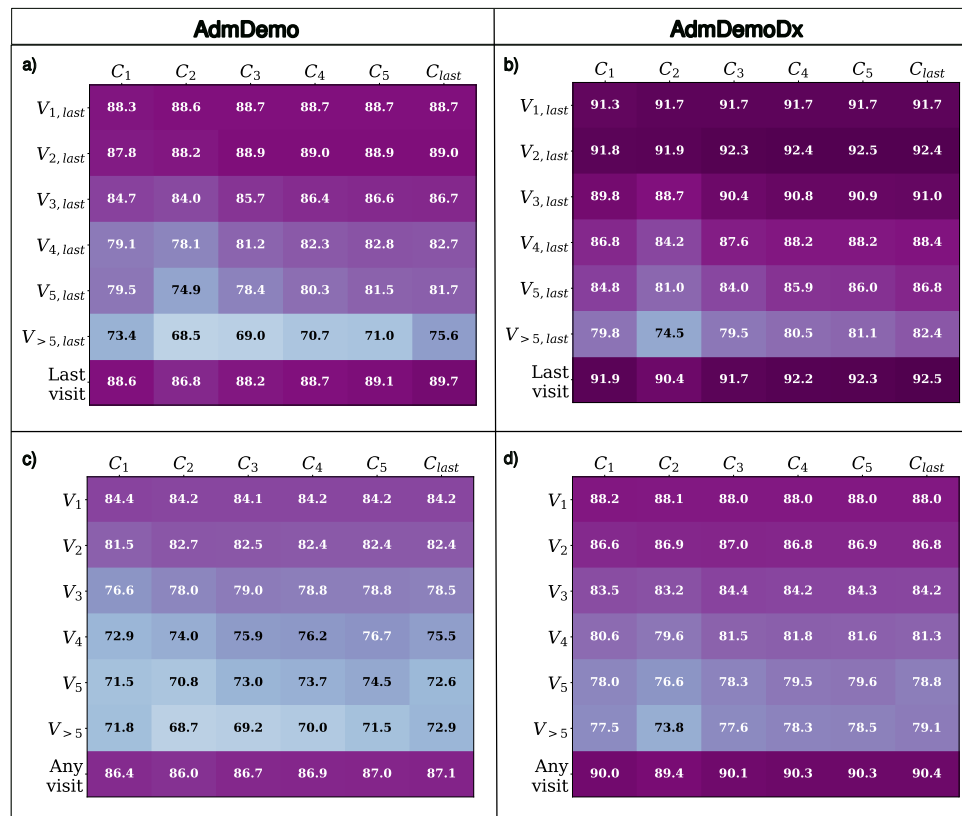
Fig. 7 Performance of each LSTM_k trained with a cohort C_k on different groups of patients. (a) and (b) Performance on the last visits of patients. (c) and (d) Performance on the last and intermediate visits of patients. The rows represent the testing patients and the columns represent the training cohorts. The scores in the intersection of a row and a column correspond to the mean of the AUROC over the 5 folds of cross-validation of an LSTM trained with the corresponding cohort and tested on the corresponding patients
