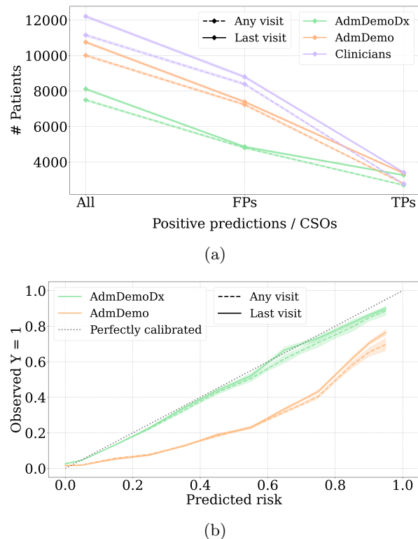
Fig. 4 Analyses of the final ELSTM tested on the holdout set with both AdmDemo and AdmDemoDx predictors. Shaded regions indicate variations within one standard deviation of the mean over 100 bootstraps. (a) Number of positive predictions by the ELSTM with AdmDemo and AdmDemoDx predictors, and CSOs documented by clinicians. The ELSTM shows a reduced number of false positives and a slight loss in the number of true positives. (b) ELSTM calibration curves with AdmDemo and AdmDemoDx predictors. We used interpolation to unify the predicted risk bins over the 100 bootstraps and generate a mean calibration curve with its variations. We show in Appendix C the 100 calibration curves for each ELSTM in the bootstrap sampling. The ELSTM-AdmDemoDx is almost identical to a perfectly calibrated model, while the ELSTM-AdmDemo tends to overestimate the risk of mortality
