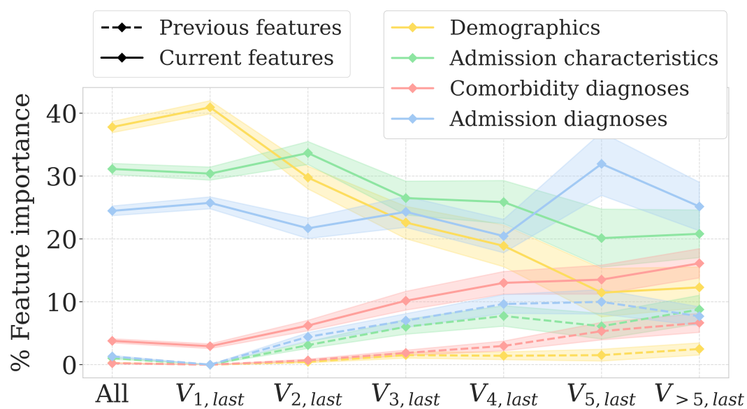
Fig. 9 Post-hoc analyses of feature importance of the ELSTM trained with AdmDemoDx predictors when including the time gap between current and previous admissions as a predictor. Importance of each feature is computed using feature permutation [26] over 100 bootstraps. Shaded regions indicate variations within one standard deviation of the mean over 100 bootstraps
