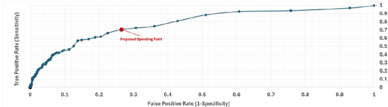
Figure 1. Classifier results showing true positive rate vs. false positive rate. The clinician-reviewed operating point is shown in red. AUC = 0.8.
