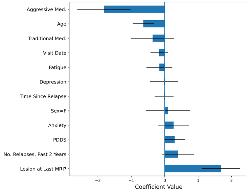
Figure 3: Logistic regression coefficients: We can assess the importance of each feature in predicting the presence of a new lesion.
