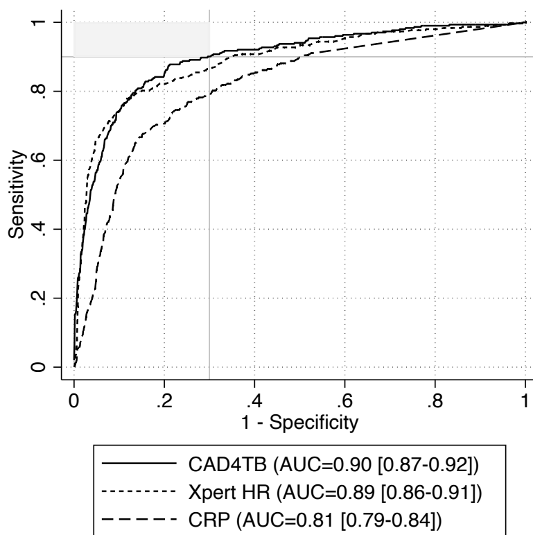
Figure 2. Receiver operating characteristic curve. ROC curves against the microbiologic reference standard with AUC and 95% CI displayed for CAD4TB, Xpert HR, and CRP. The upper-left area shaded in gray notes the region where tests meet TPP targets ( \geq 90\% sensitivity, \geq 70\% specificity). N=1,392 participants from the Philippines, Vietnam, Uganda, South Africa, and India with presumptive TB (n=303, 22% with microbiologically confirmed TB).
