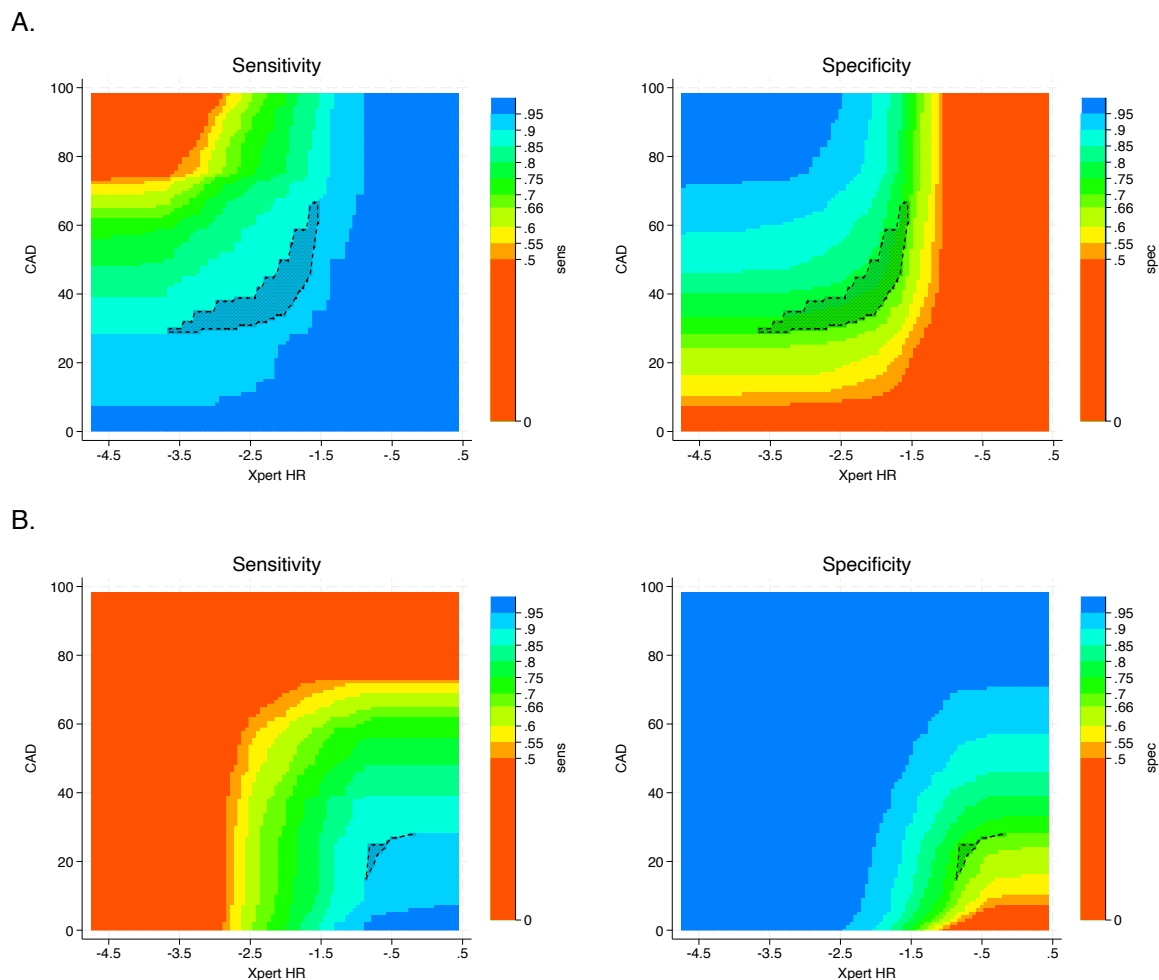
Figure 3. Selection of cut points for two-step screening algorithm combining Xpert HR and CAD4TB. Panel (A) shows the possible cut-points using sequential negative serial screening, in which the second screening test is conducted only if the first is negative and a positive screen is defined as positive on either test. Panel (B) shows the possible cut-points using sequential positive serial screening, in which the second screening test is conducted only if the first is positive and a positive screen is defined as positive on both tests. The x-axis shows all potential cut-points for Xpert HR (test positive defined as less than or equal to the cut point chosen), and the y-axis shows all potential cut points for CAD4TB (test positive defined as greater than or equal to the cut point chosen). Each point on the graph corresponds to a pair of cut points used to define a positive screening algorithm. The colors represent the range of sensitivities and specificities possible. The outlined region contains pairs with sensitivity \geq 90\% and specificity \geq 70\% ( n=417 in panel A, n=31 in panel B).
