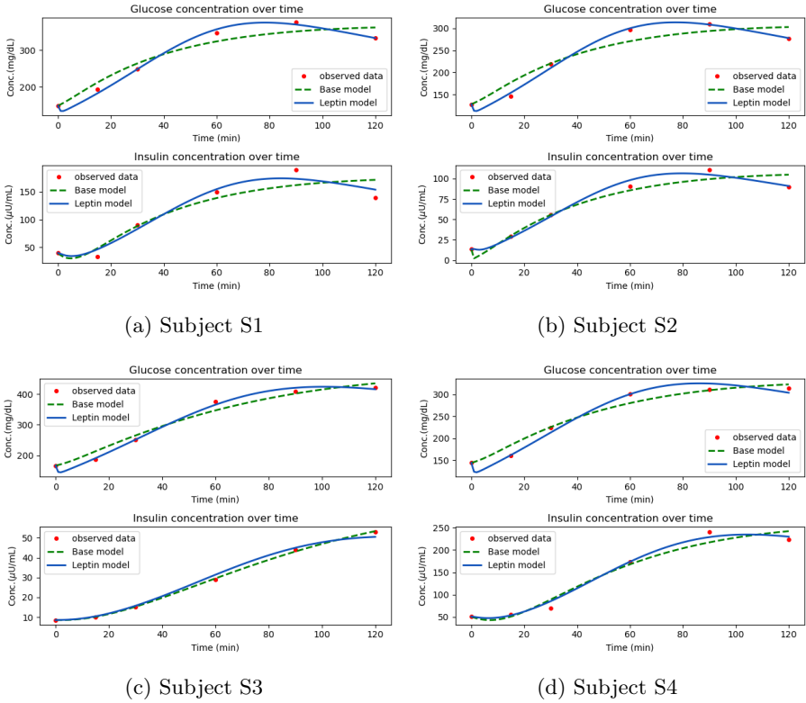
Fig. 7: Plots of sample subjects showing glucose and insulin (for 25g glucose) for base model and leptin model using dataset-II
