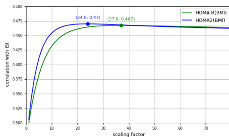
Fig. 3: Variation of scaling factor used in revised HOMA-B and HOMA2 wrt correlation with ISI
