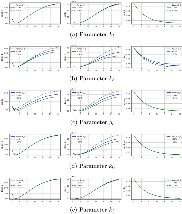
Fig. 2: Sensitivity analysis of parameters with \pm 30\% variation wrt glucose, insulin and leptin
