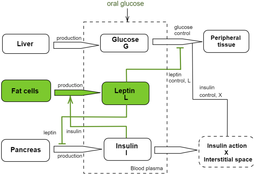
Fig. 1: Leptin model: The augmentations to the model are visually highlighted using the colour green. Leptin has glucose-lowering effects independent of insulin. Insulin increases the production of leptin by adipose tissue (fat cells). Leptin feeds back to reduce insulin secretion.
