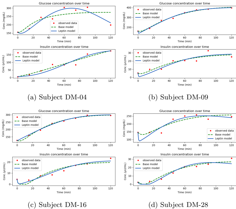
Fig. 6: Plots of sample subjects showing glucose and insulin (for 75g glucose) for base model and leptin model using dataset-I
