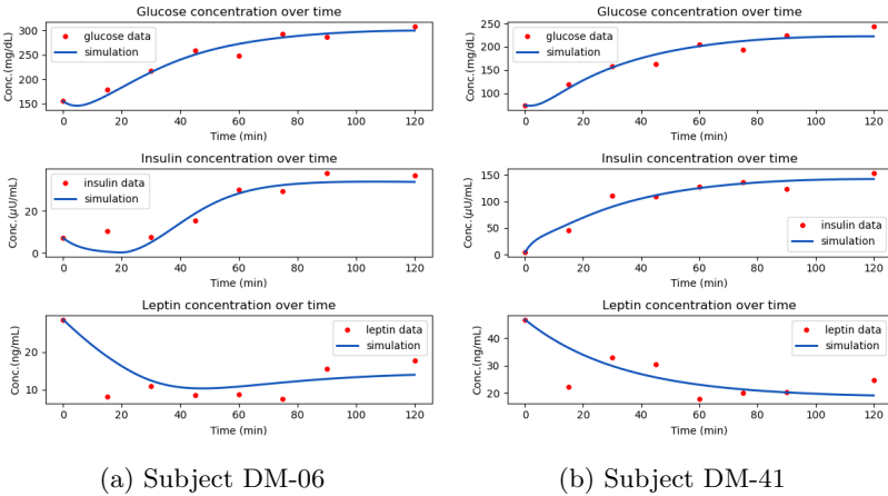
Fig. 4: Simulation results sample showing glucose, insulin and leptin concentrations for subjects
