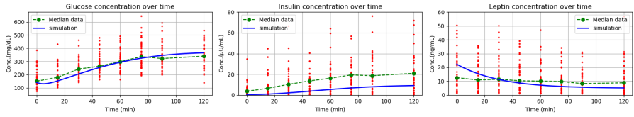
Fig. 5: Glucose, insulin, and leptin concentration range for all study participants ( n=38 ) for 2-h OGTT. Median glucose, insulin, and leptin concentrations from data (dashed green line) and simulation of leptin model (blue line) for a BMI = 25.
