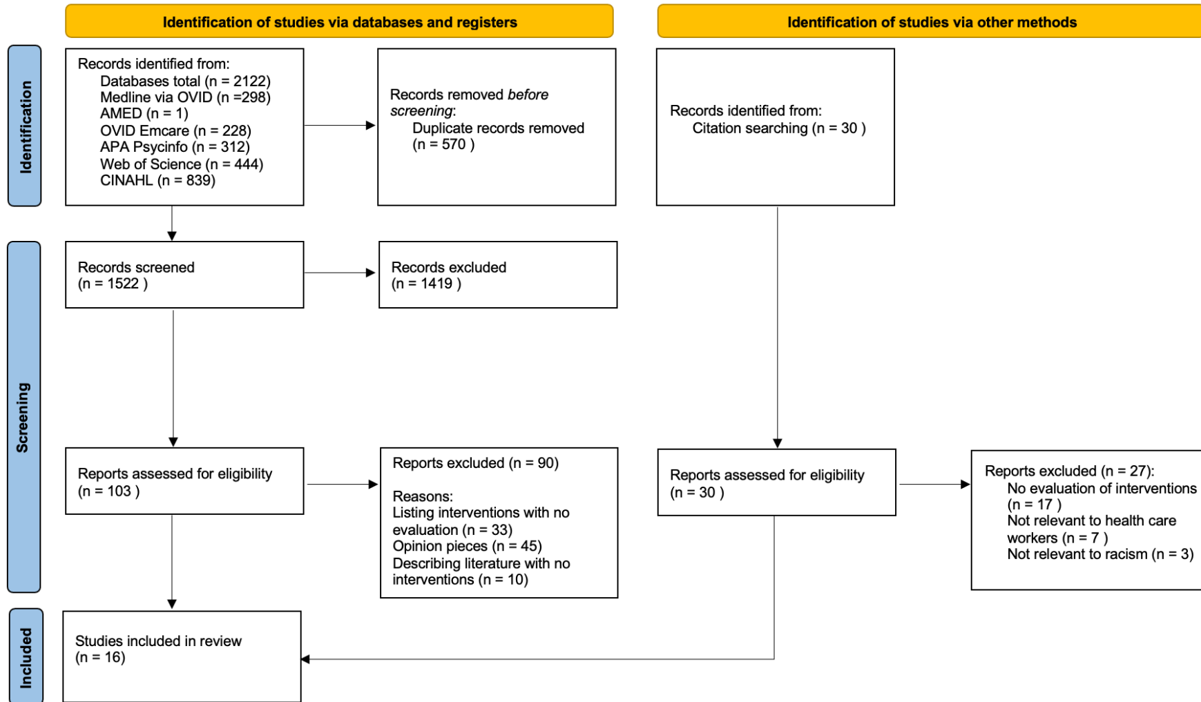
Figure 2. PRISMA Flowchart
