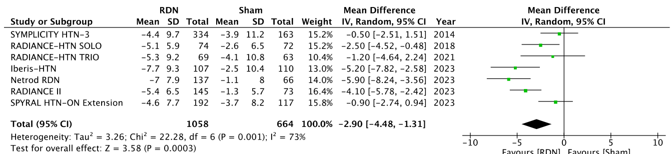
Figure 3. Comparison of effects of renal denervation vs sham procedure on daytime systolic (top forest plot) and diastolic (bottom forest plot) blood pressure
