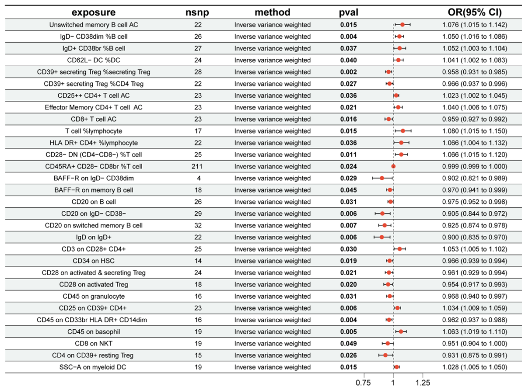
Figure 4. Forest plot for 30 immunophenotypes correlated with LC. MVMR study utilizing 731 immune cell phenotypes as exposures to investigate their potential causal effects on LC. 30 phenotypes were identified as significantly associated with LC. The OR and 95% CI for these associations are presented.
