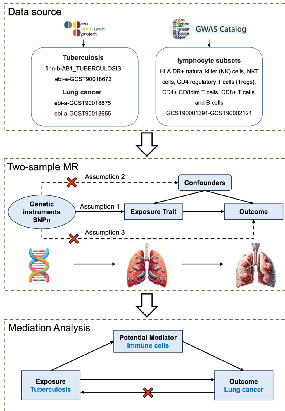
Figure 1. Overview of MR assumptions. MR study rationale: assumption 1, Genetic instruments must be associated with the exposure.; assumption 2, Genetic instruments must not be associated with any confounders.; assumption 3, Genetic instruments must not be directly associated with the outcome; they should influence the outcome solely through their impact on the exposure.
