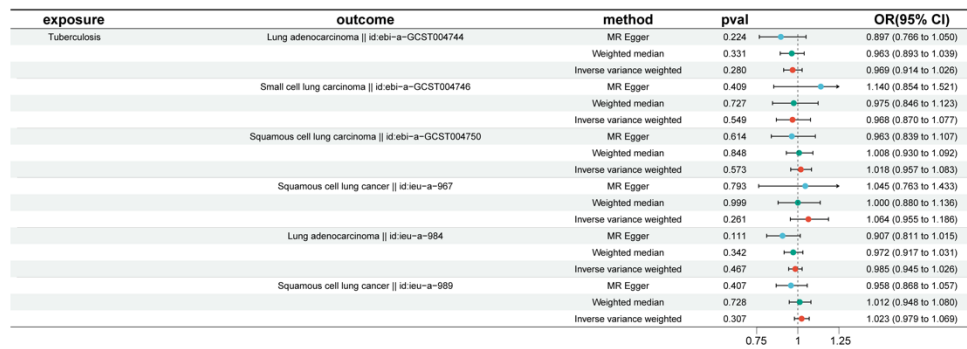
Figure 3. MR analyses of TB and LC with different pathological subtypes.
