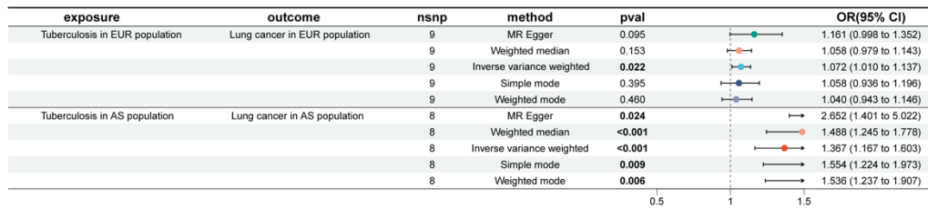
Figure 2. MR analyses of TB and LC. MR analyses demonstrate the causal effect of TB on LC in European and Asian populations using five methods: MR Egger, weighted median, IVW, simple mode, and weighted mode. OR, 95% CI, and P -values are shown for each method.
