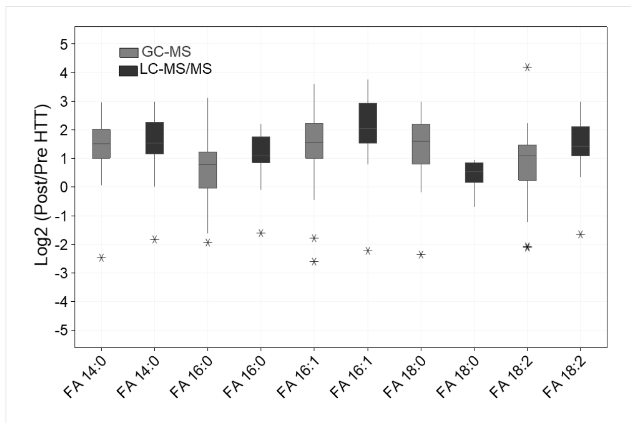
536 537 Figure S1. Cross-validation of fatty acids by LC-MS/MS and GC-MS. To confirm the 538 fatty acid profiles observed by liquid chromatography-tandem mass spectrometry (LC- 539 MS/MS), we performed gas chromatography-mass spectrometry (GC-MS) analysis, 540 which showed similar fold change profiles.
