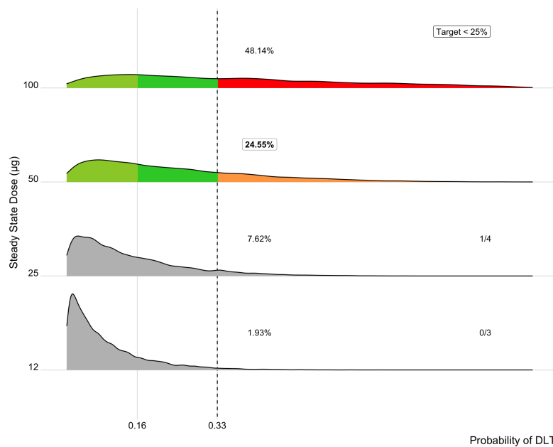
Fig. 1 Posterior densities after 1 DLT observed out of 4 subjects in the second regimen, and 0 DLTs observed out of 3 subjects in the first regimen. Red colour indicates that the probability mass \geq 0.33 is > 0.25 .
