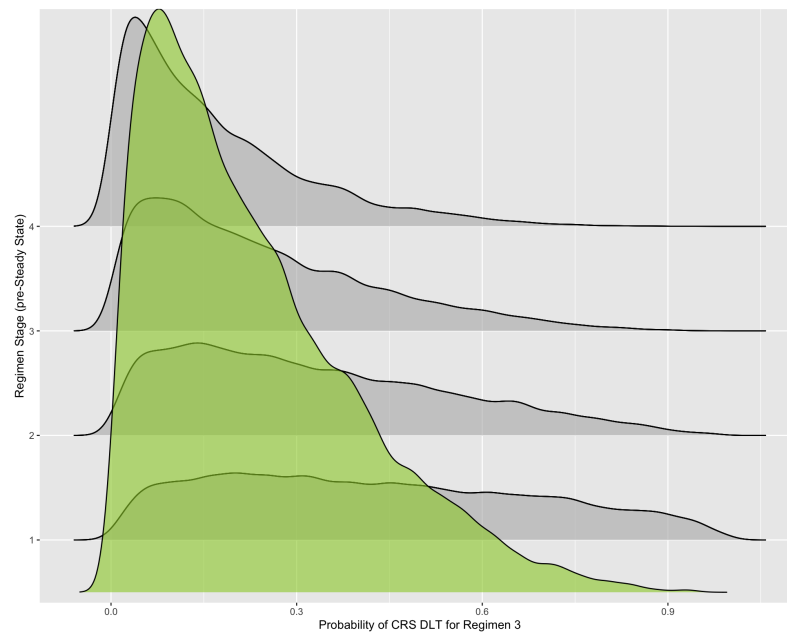
Fig. 2 Posterior densities (grey) contributing to overall posterior probability (green) of CRS for DR3.
