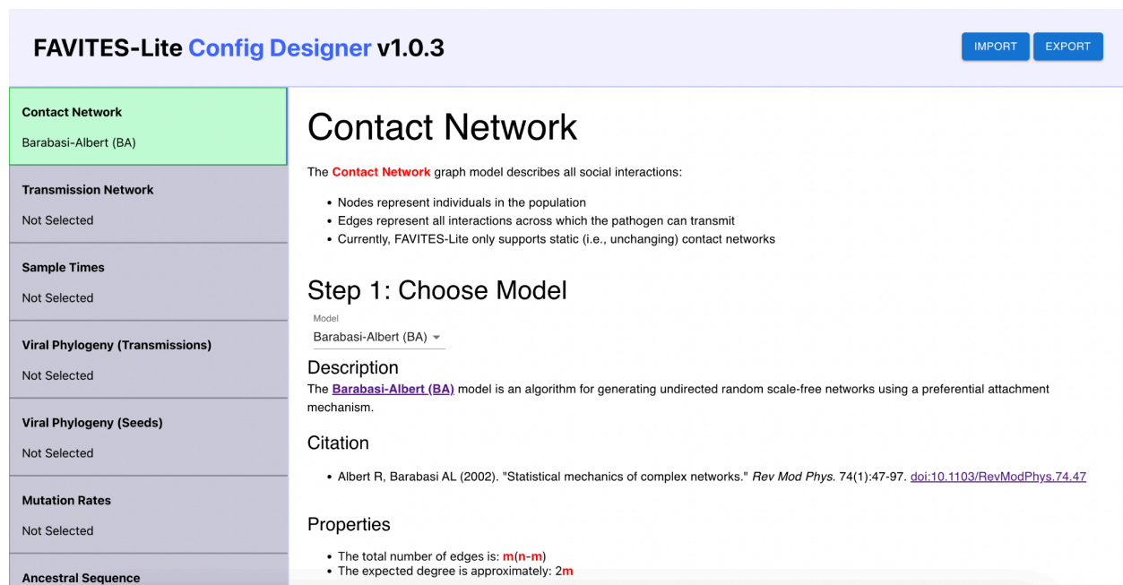
Figure 1: Screenshot of the FAVITES-Lite Config Designer web application.
