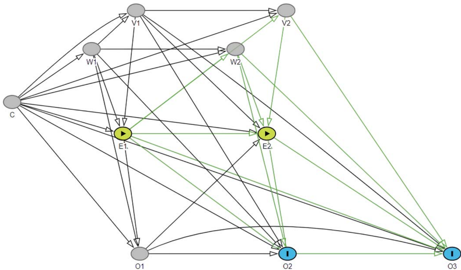
Figure 3. An alternative DAG. E is the exposure of interest; O is the outcome; C represents time-fixed confounders; W and V represent time-varying confounders affecting with and without lag (W) or only with lag (V). Numbers (1, 2 or 3) refer to time point. Green paths are causal paths from exposure to outcomes of interest.
