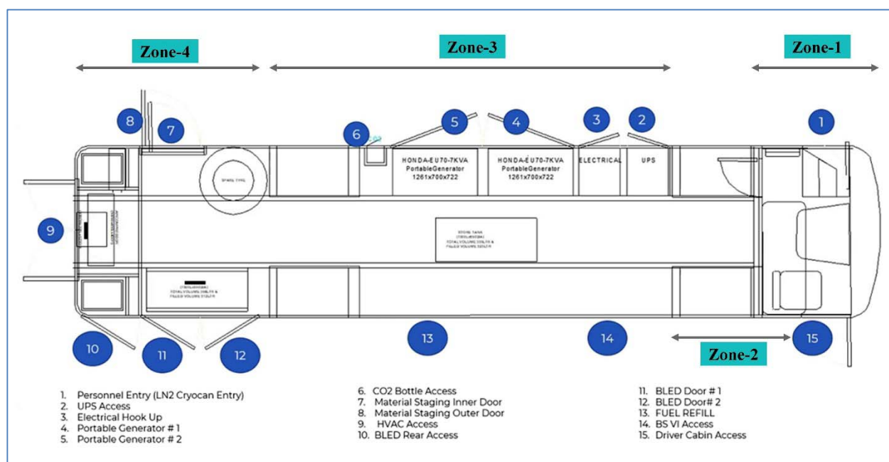
Figure 1: Zone-wise layout of the MBSL-3 laboratory
