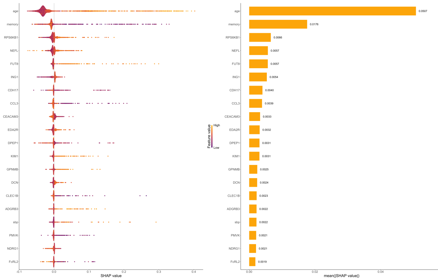
A) SHapley Additive exPlanations (SHAP) values from eXtreme Gradient Boosting (XGBoost) model displaying the selected features. The y-axis indicates the feature names in order of importance ranked from top to bottom. The x-axis represents the SHAP value, which indicates the degree of change in log odds. The width of the range of the horizontal bars showed the extent of the contribution to the prediction of all-cause dementia. The color of each point on the graph represents the value of the corresponding feature, with orange indicating high values and purple indicating low values. The direction on the x-axis indicates the likelihood of developing all-cause dementia towards the right, and likelihood of free from dementia towards the left. B) Mean absolute SHAP values for each feature derived from XGBoost model.
