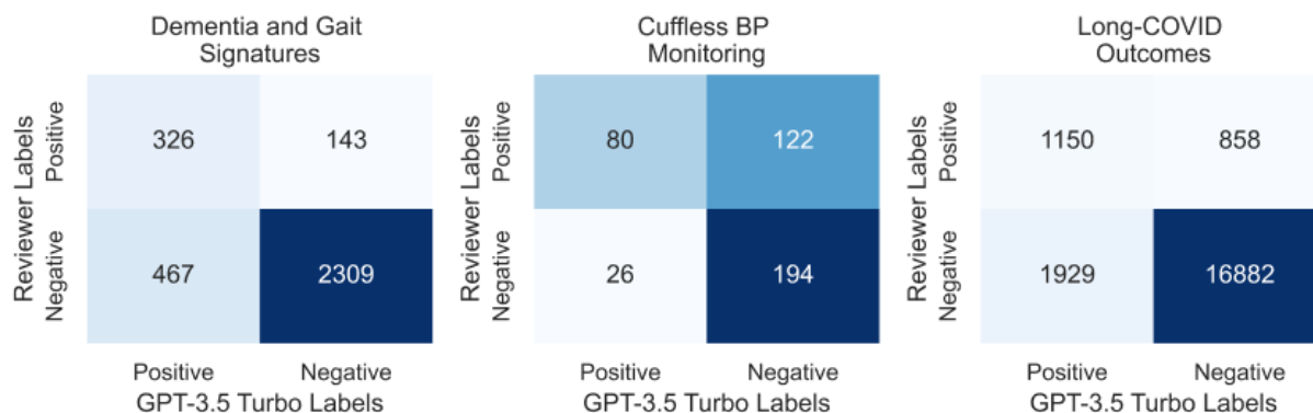
Figure 1. Alignment of Model Predictions with Human Reviewers: Confusion Matrices Comparing GPT-3.5 Turbo Decisions Against Reviewer Judgments for Title-Abstract Screening Tasks in Dementia Gait, Cuffless Blood Pressure Monitoring, and Long-COVID Studies.
