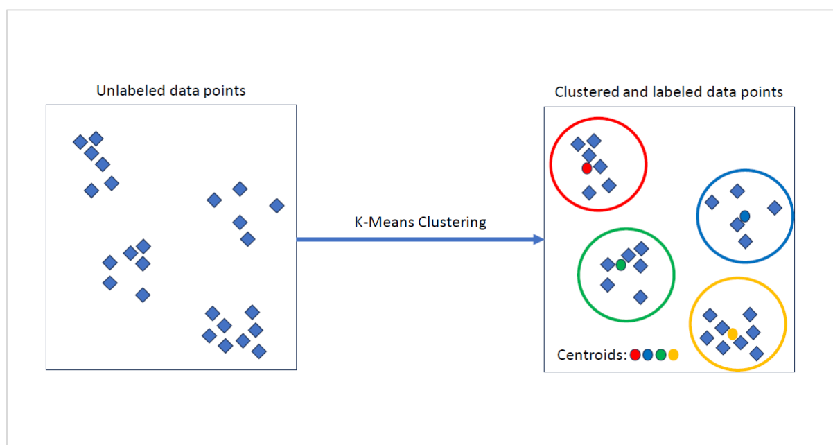
Figure 1. K-means clustering
