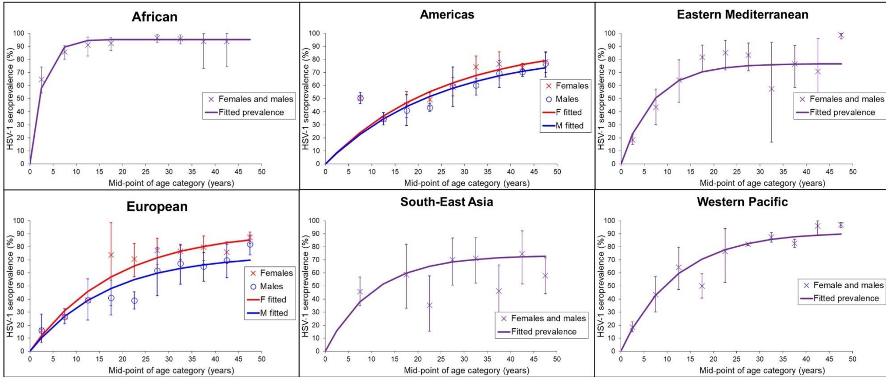
Figure S2. Model fits for HSV-1 prevalence (any site; oral and genital) for each WHO region.
