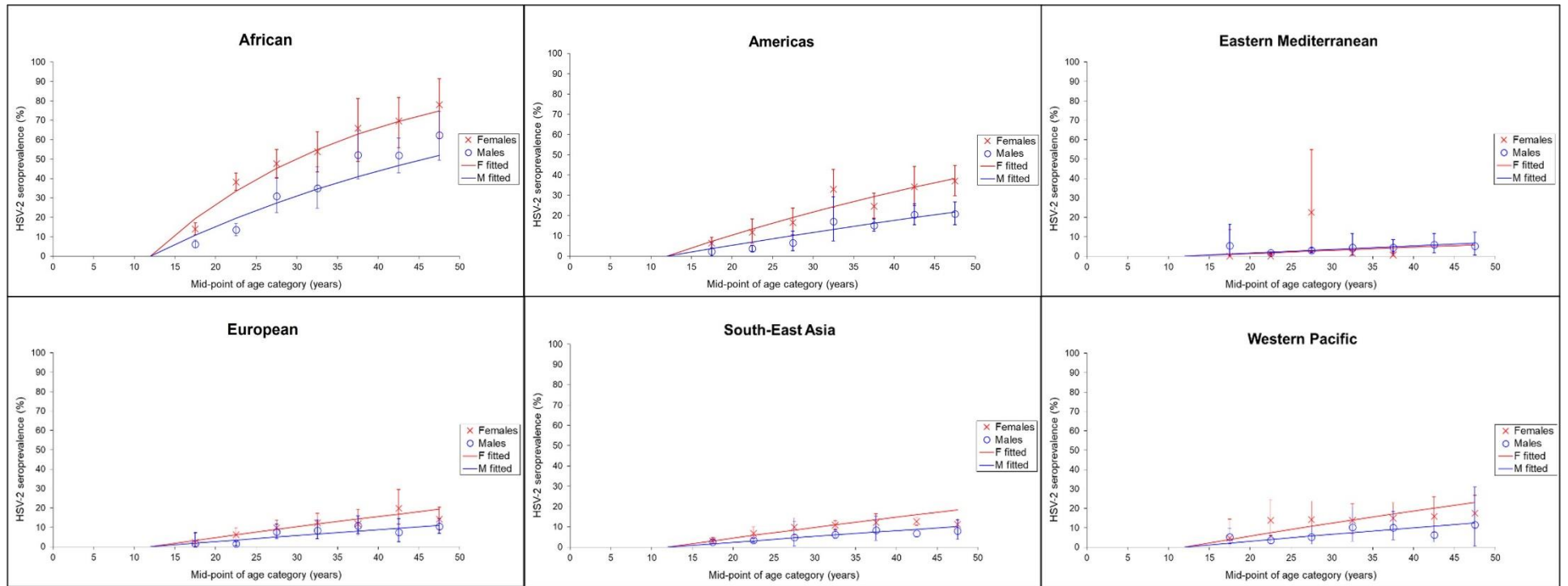
Figure S1. Model fits for HSV-2 prevalence for each WHO region.
