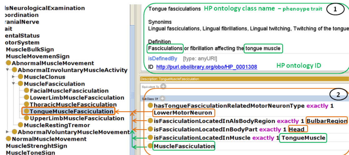
Fig. 2. The definition of the class Tongue Muscle Fasciculation in DALSO (screenshot from ontology editor Protege-2000). On the left, a fragment of class hierarchy, defined class highlighted in orange. Green panel (1), references from HP ontology to the class Tongue Muscle Fasciculation: HP term for a phenotype trait, HP identifier and textual definition. Orange panel (2), details of the class Tongue Muscle Fasciculation definition. Notions implicitly present in HP definition, Tongue Muscle and Fasciculation (marked with green) are made explicit, additional notions Lower Motor Neuron , Bulbar Region and Head are also made explicit (marked with orange). The resulting definition of Tongue Fasciculation in DALSO allows for deeper understanding of modeled phenotype trait.
