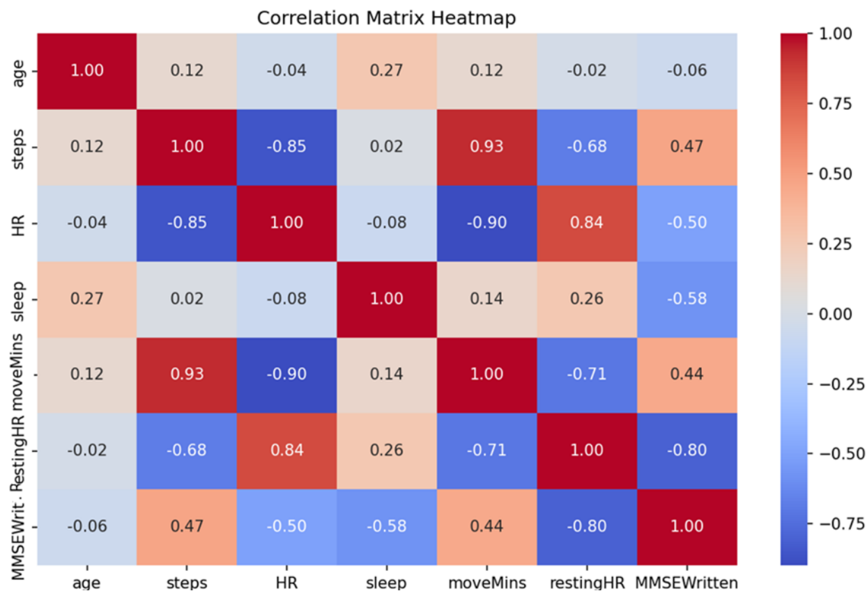
Figure 5 Correlation coefficient heatmap of all continuous variables show that number of steps and number of minutes of movement are significantly positively correlated with higher MMSE score with p-value \leq 0.05 . Resting HR Rate is negatively correlated with higher MMSE score with p-value of 0.007
