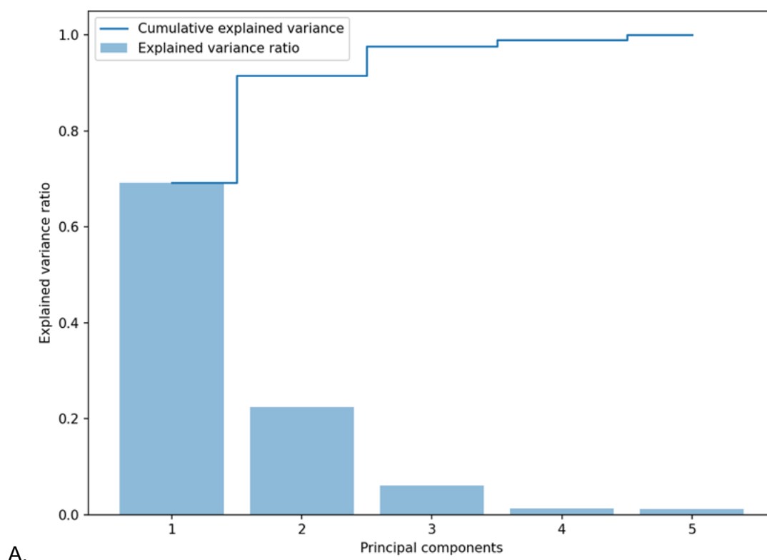
Figure 4 (A) Cumulative Explained Variance and Explained Variance Ratio (B) Top two dimensions of the PCA analysis based on the smart wristband health data variables of patients show the spread between the patients with higher cognitive scores (MMSE \geq 25) cluster together and away from the patients with lower cognitive scores (MMSE < 25) (C) Gender distribution in top two dimensions (D) Age distribution in top two dimensions (E) Eigenvectors of the first five principal components show that sleep is the highest negative contributor and Steps and Move minutes are the highest positive contributor to the cognitive test
