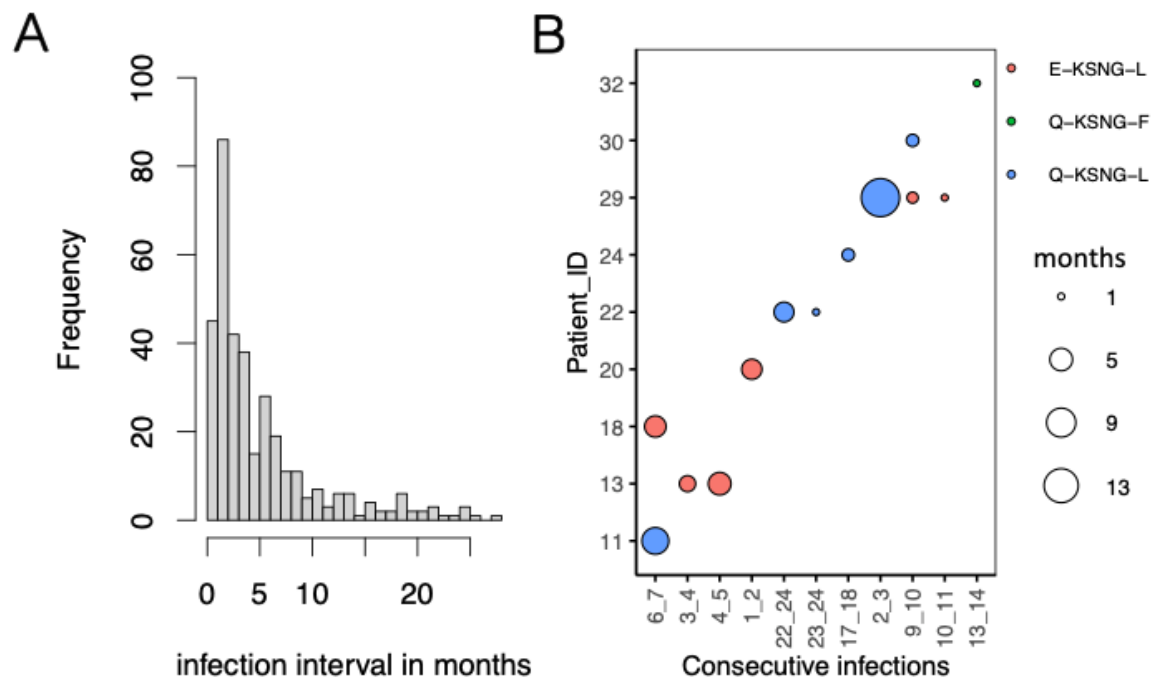
365 366 367 368 Figure 3: Distribution of infection intervals. (A) Frequency histogram of the distribution of the time interval 369 between infections in months for all infections with genotype data. (B) Interval in months for individuals 370 with consecutive infections of the same microhaplotype. The size of the circles depicts the number of 371 months between infections with the same microhaplotype depicted by the color of the circle.
