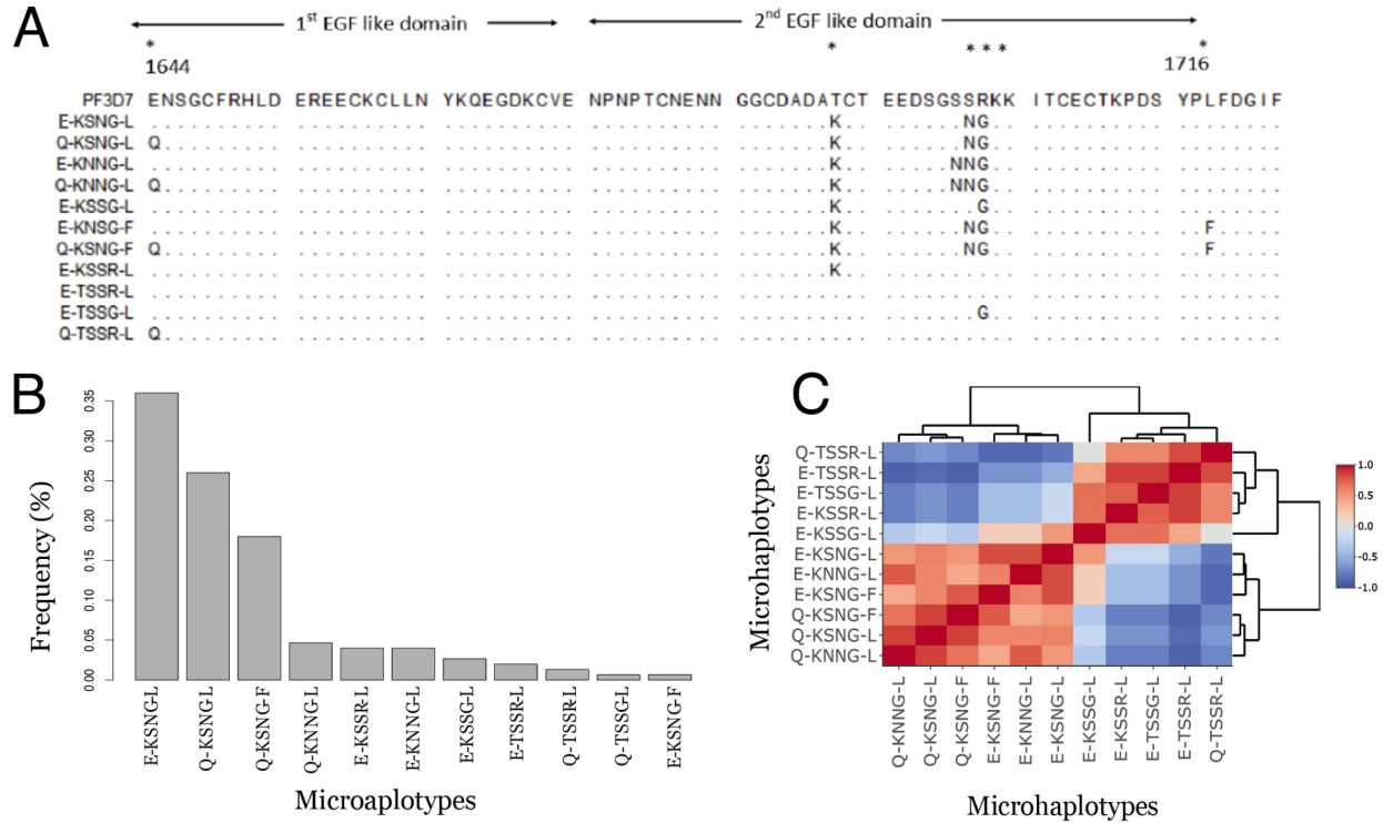
343 Figure 1. Dynamics of P. falciparum msp1 19 microhaplotypes. (A) Amino- acid sequence alignment of 11 344 identified microhaplotypes. Polymorphic sites are shown with an asterisk (*). The nucleotide positions 345 relative to the start position of the Pfmsp1 gene are shown below the asterisk. The dots in the alignment 346 indicate the position corresponding to P. falciparum 3D7 with identical amino acid sequences. The 347 epidermal growth factor (EGF)-like domains 1 and 2 are shown by arrows. The first polymorphism is 348 located in the first EGF-like domain, whereas the second to the fifth polymorphism are located in the 349 second EGF-like domain. (B) Microhaplotypes sorted by their abundance in the population. (C) 350 Microhaplotypes clustered to groups based on the number of nucleotide differences between haplotypes. 351 The dendrogram on the sides of the heatmap visually represents the relatedness of the microhaplotypes. 352 In this context, the branches indicate distinct clusters formed through hierarchical clustering, highlighting 353 groups of haplotypes with similar characteristics. Scale=Pearson correlation coefficients.
