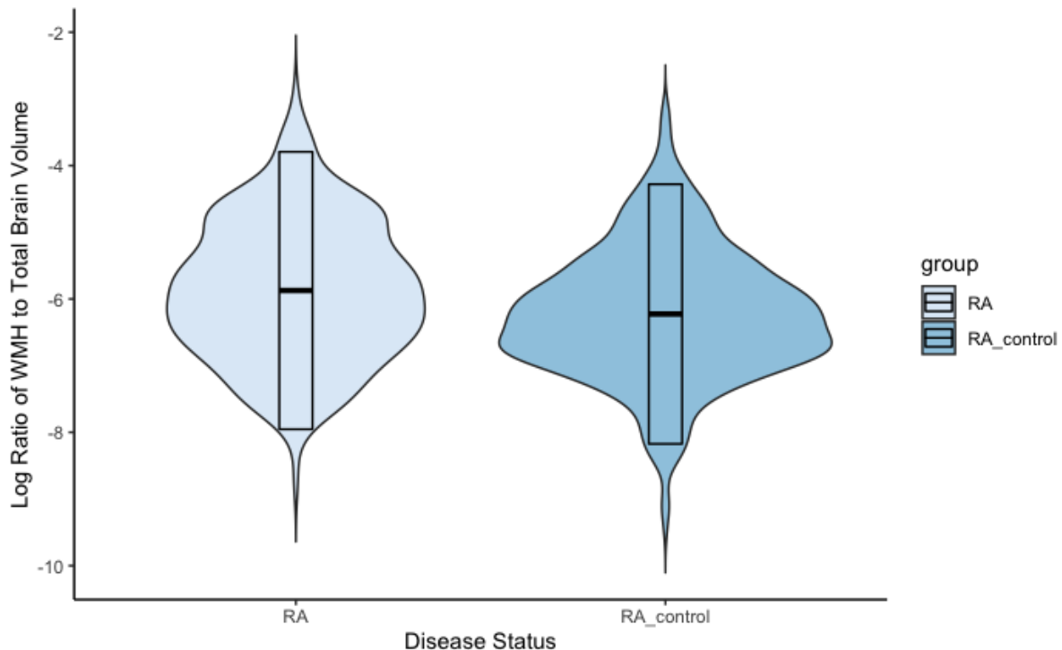
Figure 2 Violin plot representing the log transformed ratio of the total volume of white matter hyperintensities to total brain volume in patients with rheumatoid arthritis as compared to a matched control group.
