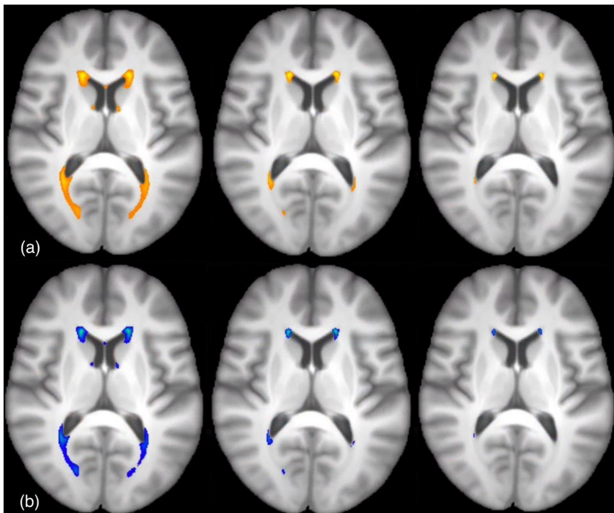
Figure 4 Average lesion maps representing lesion distribution in (a) RA patients (yellow) (b) UC patients (blue) thresholded from left to right at 5%, 50% and 70%.
