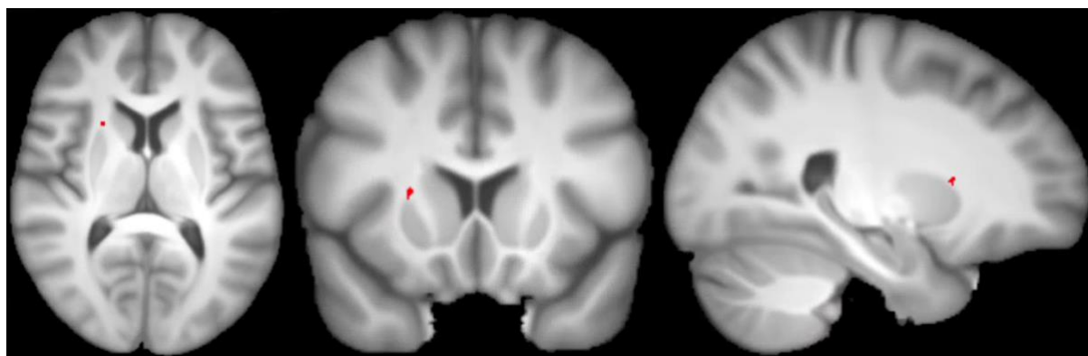
Figure 5: Threshold free cluster enhancement results from voxel wise analysis of RA subjects compared to age, sex and total volume of white matter hyperintensities matched controls. MNI coordinates 24 x 15 x 9.
