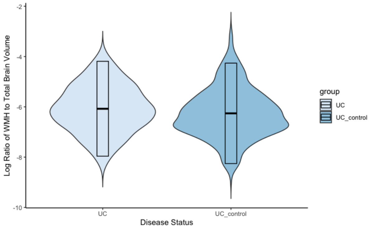
Figure 3 Violin plot representing the log transformed total volume of white matter hyperintensities to total brain volume in patients with ulcerative colitis as compared to a matched control group.
