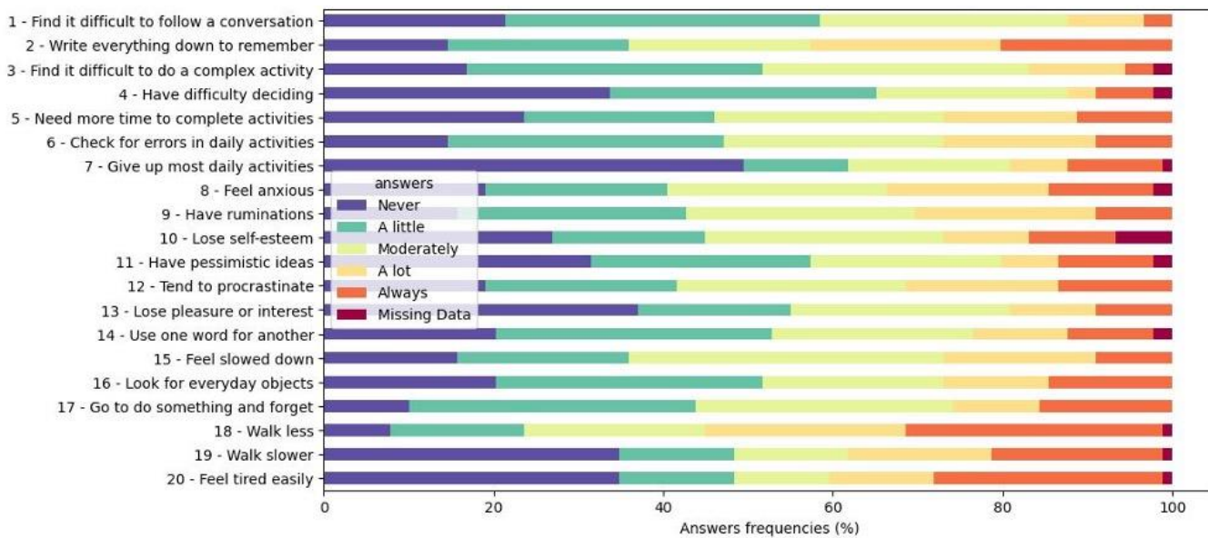
Figure 1: Frequencies of answers obtained at inclusion visit for the selection of items composing the validation-study version of the CADA-PRO tool (N=89)
