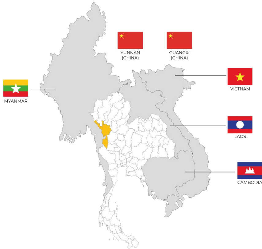
114 Figure 1: A map of the Greater Mekong Subregion (GMS) with the sample site highlighted in 115 Mae Sot District, Tak Province, Thailand.
