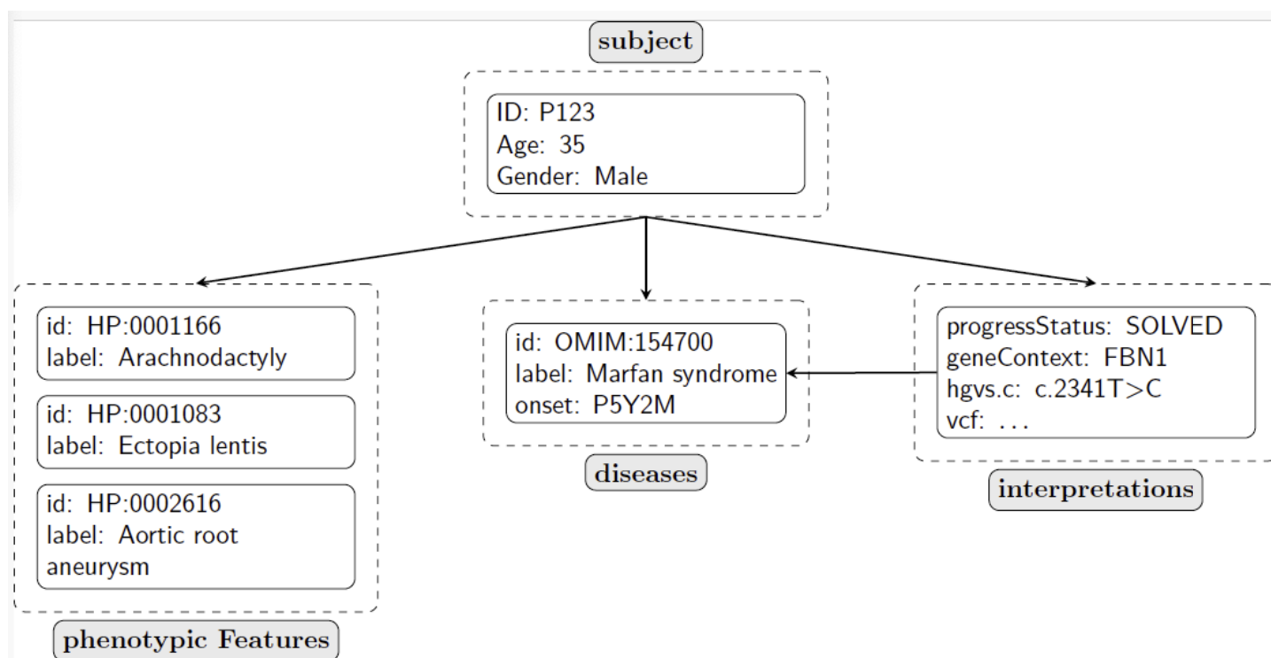
Figure 2 -- Schematic visualization of a phenopacket. In this simplified representation, the major elements of the Phenopacket Schema used for the Phenopackets in this collection are shown. The subject of the phenopacket is represented using the Individual element, which allows the (anonymous) identifier, age at last examination, and sex to be specified. Each subject can have an arbitrary number of phenotypic features, which comprise an HPO term and optionally information about the age of onset of the feature. The subject can have an arbitrary number of diseases, but for the phenopackets contained in this collection, each subject has one disease. The subject can have an arbitrary number of interpretations, which must refer to a disease in the disease list. In this example, a pathogenic variant in the FBN1 gene is interpreted to be causal for Marfan syndrome.
