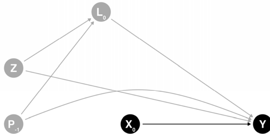
Figure 1: Causal directed acyclic graph (DAG) depicting confounding (A) and successful emulation of randomization using g methods (B) at baseline between the intervention strategy ( X ) and outcome ( Y ). Baseline covariates (both time-invariant [ Z ] and time-varying [ L ]) as well as prior diet and physical activity habits ( P ) must be considered to emulate randomization. The successful emulation of randomization of the lifestyle intervention strategy requires no unmeasured confounders and no residual confounding. Time-varying treatment and covariates are not shown in this DAG to focus on randomization emulation.
