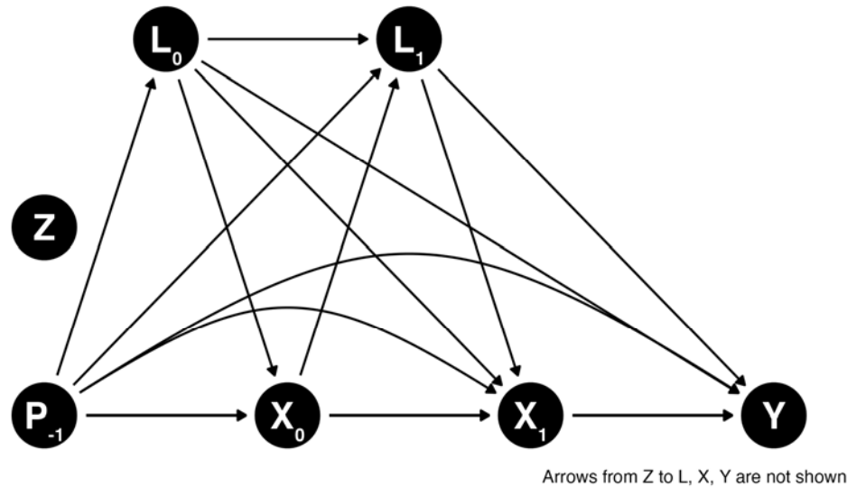
Figure 2: Directed acyclic graph (DAG) depicting the hypothesized relationship among prior dietary exposure and time-varying interventions (diet, physical activity) and covariates. Arrows from the Z node are not shown for clarity, but would point towards all baseline and time-varying nodes, as well as outcome. Only one follow-up is shown for visualization purpose, but the hypothesized causal structure extends to additional follow-ups.
