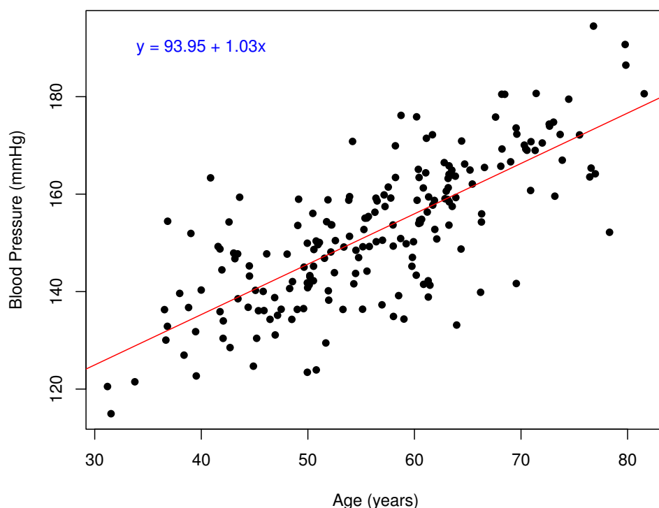
Figure 1. Example data on age and blood pressure and the line from a linear regression model.
