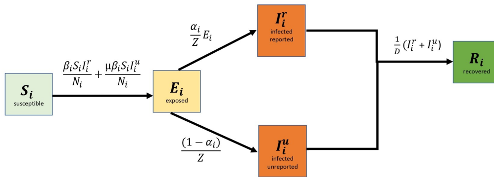
Figure 1: Schematic presentation of simulated disease dynamics. The solid arrows demonstrate the movement from one disease state to another.
